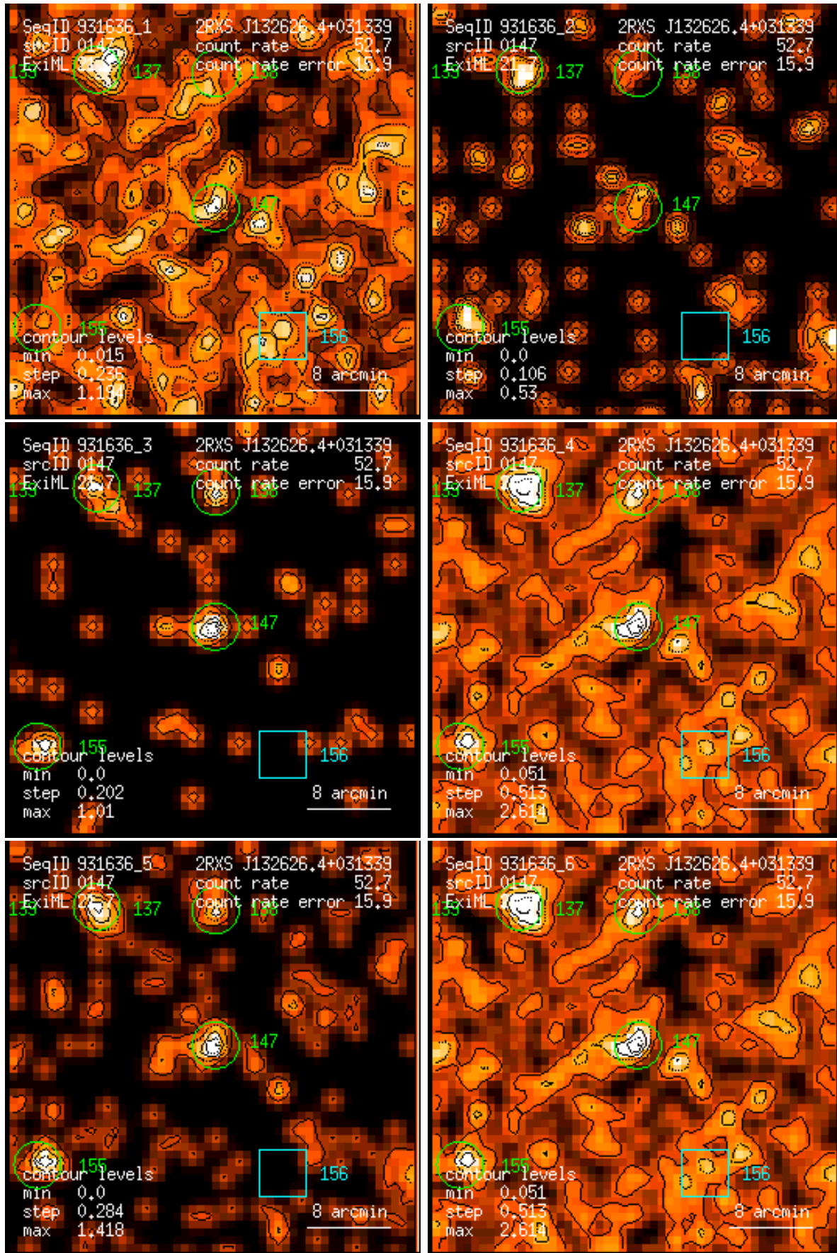
Figure 147: RASS 931636: detection 0147: band rate images, Gaussian filter: (1) PSPC channels 11 – 41, (2) 52 – 90, (3) 91 – 201, (4) 11 – 235, (5) 52 – 201, (6) 11 – 201. Broad band rates in counts/ks. Band rate contour levels in counts/ks/arcmin 2 .
