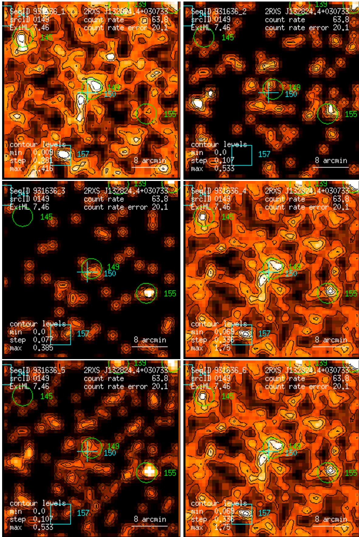
Figure 149: RASS 931636: detection 0149: band rate images, Gaussian filter: (1) PSPC channels 11 – 41, (2) 52 – 90, (3) 91 – 201, (4) 11 – 235, (5) 52 – 201, (6) 11 – 201. Broad band rates in counts/ks. Band rate contour levels in counts/ks/arcmin 2 .
