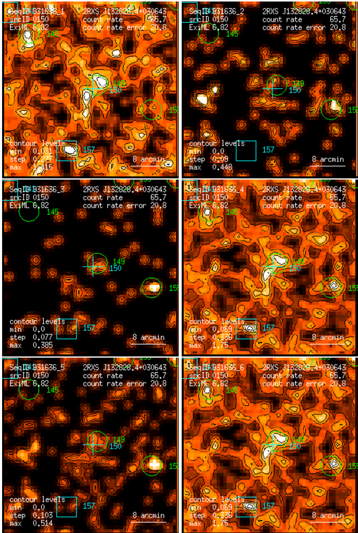
Figure 150: RASS 931636: detection 0150: band rate images, Gaussian filter: (1) PSPC channels 11 – 41, (2) 52 – 90, (3) 91 – 201, (4) 11 – 235, (5) 52 – 201, (6) 11 – 201. Broad band rates in counts/ks. Band rate contour levels in counts/ks/arcmin 2 .
