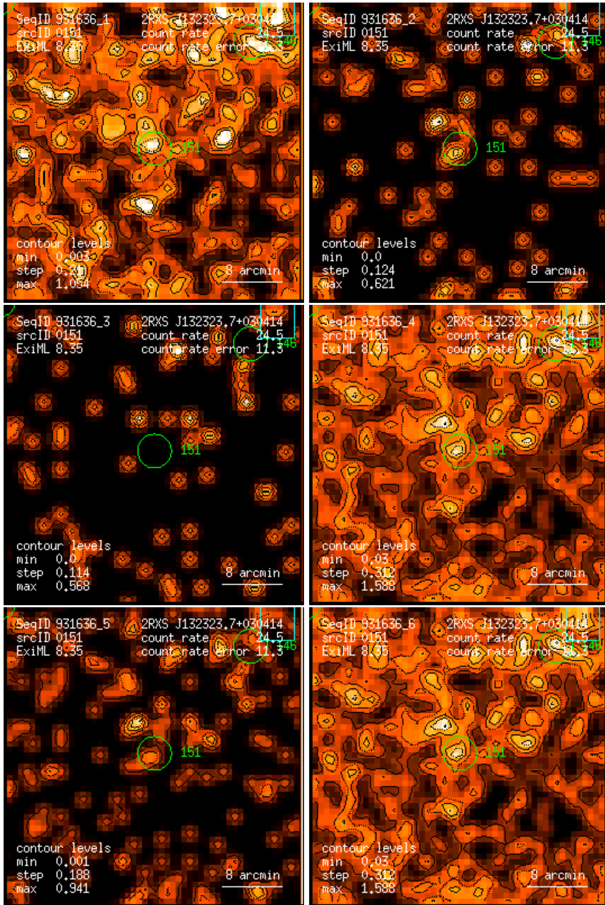
Figure 151: RASS 931636: detection 0151: band rate images, Gaussian filter: (1) PSPC channels 11 – 41, (2) 52 – 90, (3) 91 – 201, (4) 11 – 235, (5) 52 – 201, (6) 11 – 201. Broad band rates in counts/ks. Band rate contour levels in counts/ks/arcmin 2 .
