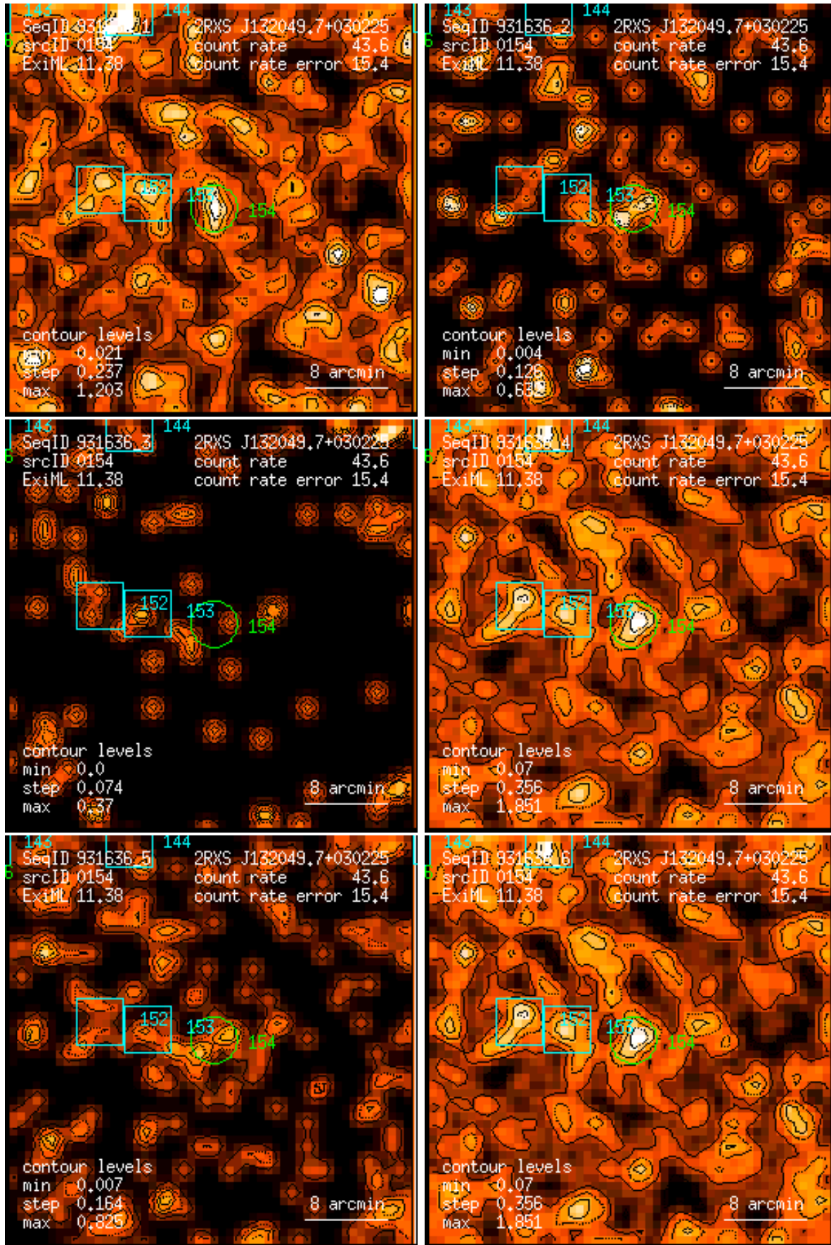
Figure 154: RASS 931636: detection 0154: band rate images, Gaussian filter: (1) PSPC channels 11 – 41, (2) 52 – 90, (3) 91 – 201, (4) 11 – 235, (5) 52 – 201, (6) 11 – 201. Broad band rates in counts/ks. Band rate contour levels in counts/ks/arcmin 2 .
