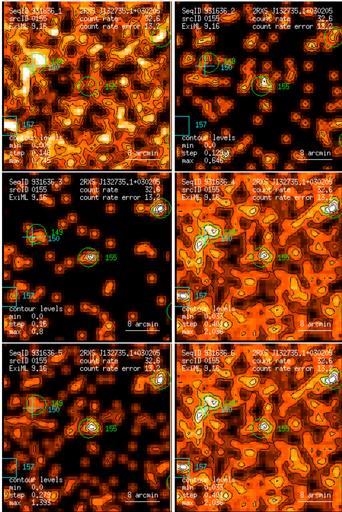
Figure 155: RASS 931636: detection 0155: band rate images, Gaussian filter: (1) PSPC channels 11 – 41, (2) 52 – 90, (3) 91 – 201, (4) 11 – 235, (5) 52 – 201, (6) 11 – 201. Broad band rates in counts/ks. Band rate contour levels in counts/ks/arcmin 2 .
