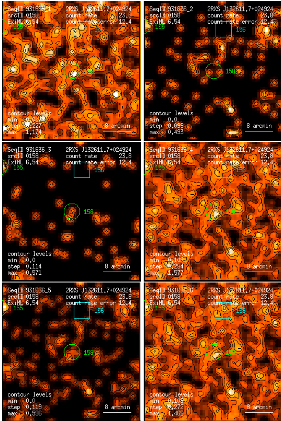
Figure 158: RASS 931636: detection 0158: band rate images, Gaussian filter: (1) PSPC channels 11 – 41, (2) 52 – 90, (3) 91 – 201, (4) 11 – 235, (5) 52 – 201, (6) 11 – 201. Broad band rates in counts/ks. Band rate contour levels in counts/ks/arcmin 2 .
