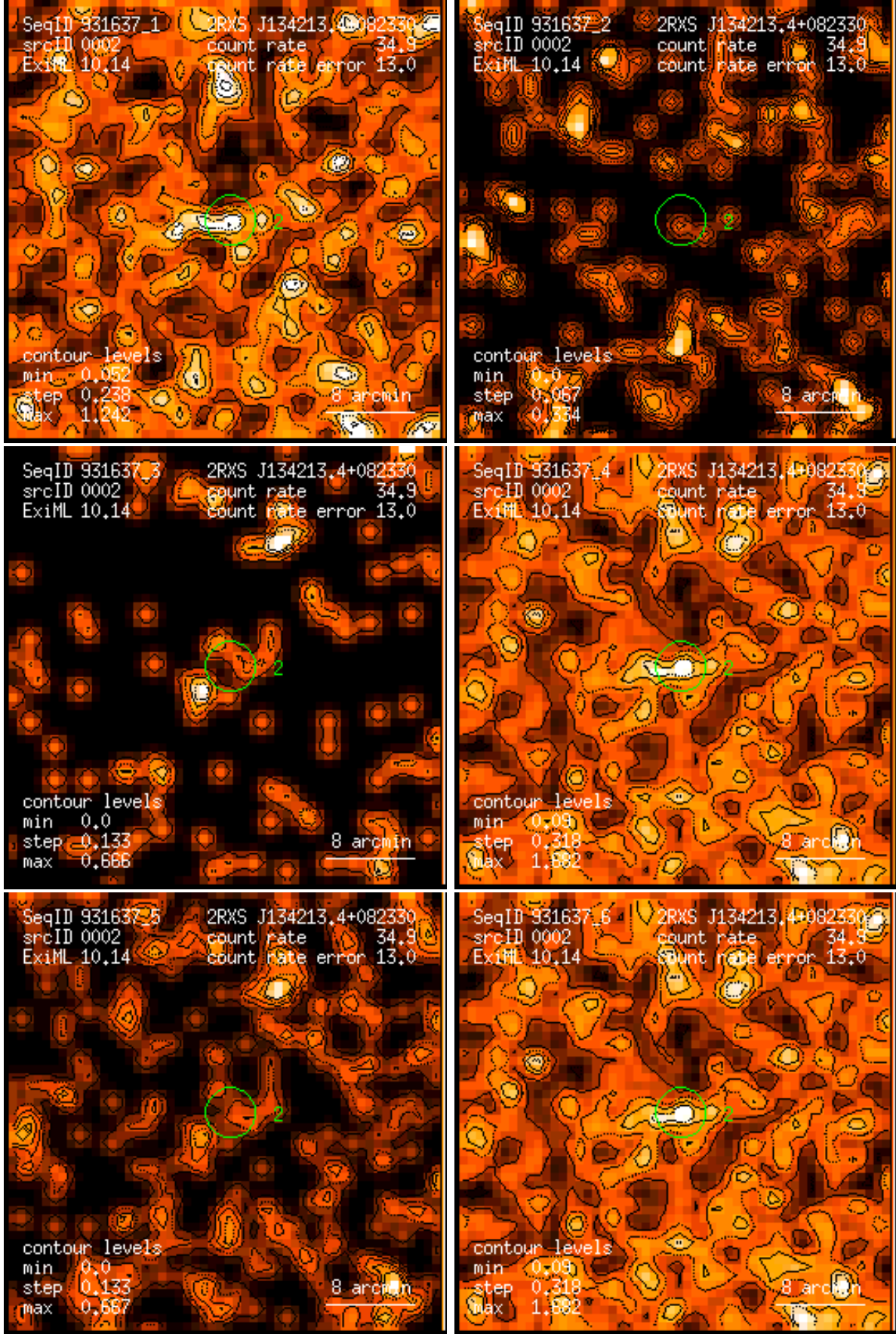
Figure 2: RASS 931637: detection 0002: band rate images, Gaussian filter: (1) PSPC channels 11 – 41, (2) 52 – 90, (3) 91 – 201, (4) 11 – 235, (5) 52 – 201, (6) 11 – 201. Broad band rates in counts/ks. Band rate contour levels in counts/ks/arcmin 2 .
