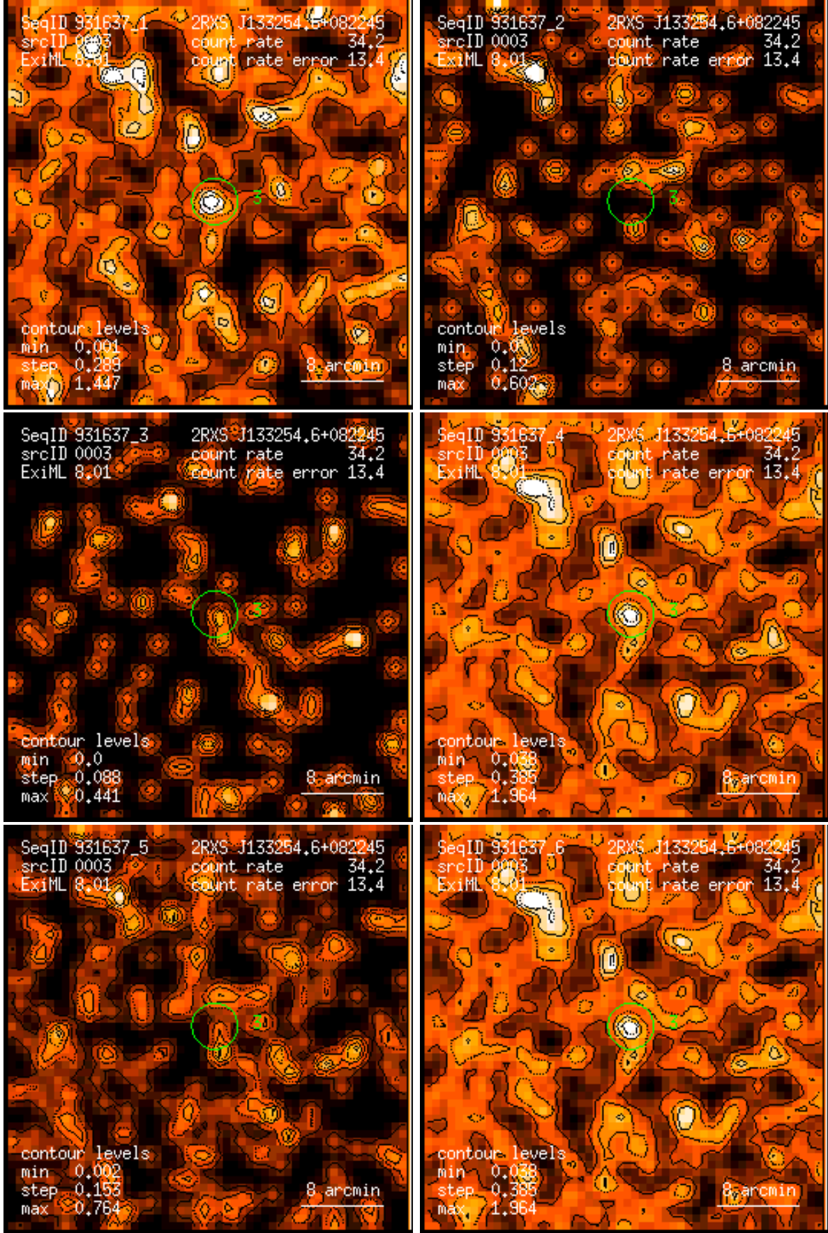
Figure 3: RASS 931637: detection 0003: band rate images, Gaussian filter: (1) PSPC channels 11 – 41, (2) 52 – 90, (3) 91 – 201, (4) 11 – 235, (5) 52 – 201, (6) 11 – 201. Broad band rates in counts/ks. Band rate contour levels in counts/ks/arcmin 2 .
