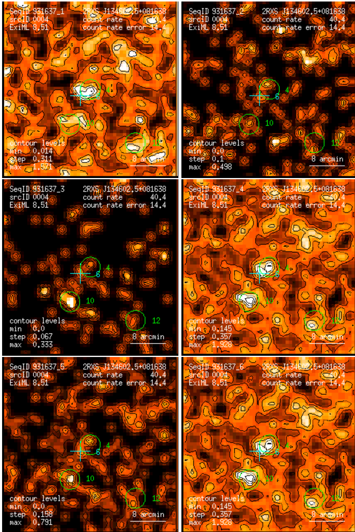
Figure 4: RASS 931637: detection 0004: band rate images, Gaussian filter: (1) PSPC channels 11 – 41, (2) 52 – 90, (3) 91 – 201, (4) 11 – 235, (5) 52 – 201, (6) 11 – 201. Broad band rates in counts/ks. Band rate contour levels in counts/ks/arcmin 2 .
