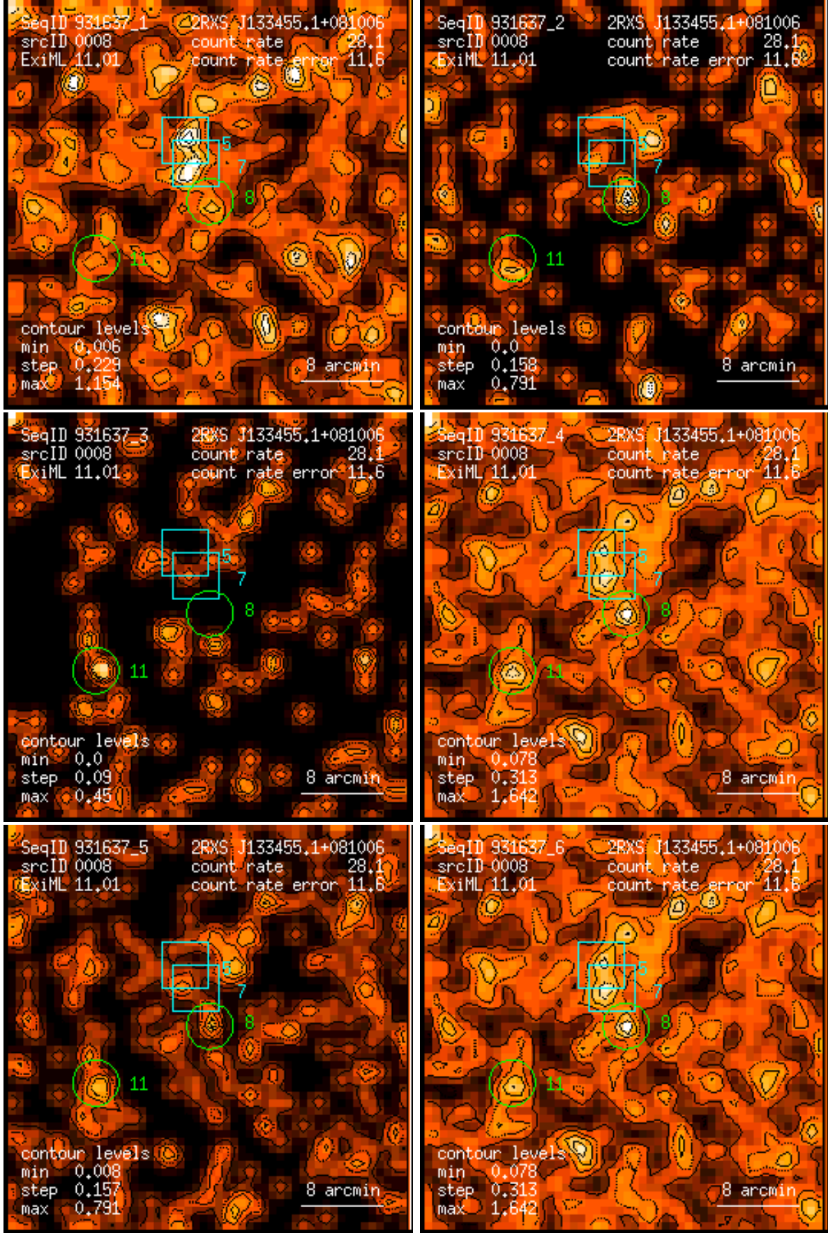
Figure 8: RASS 931637: detection 0008: band rate images, Gaussian filter: (1) PSPC channels 11 – 41, (2) 52 – 90, (3) 91 – 201, (4) 11 – 235, (5) 52 – 201, (6) 11 – 201. Broad band rates in counts/ks. Band rate contour levels in counts/ks/arcmin 2 .
