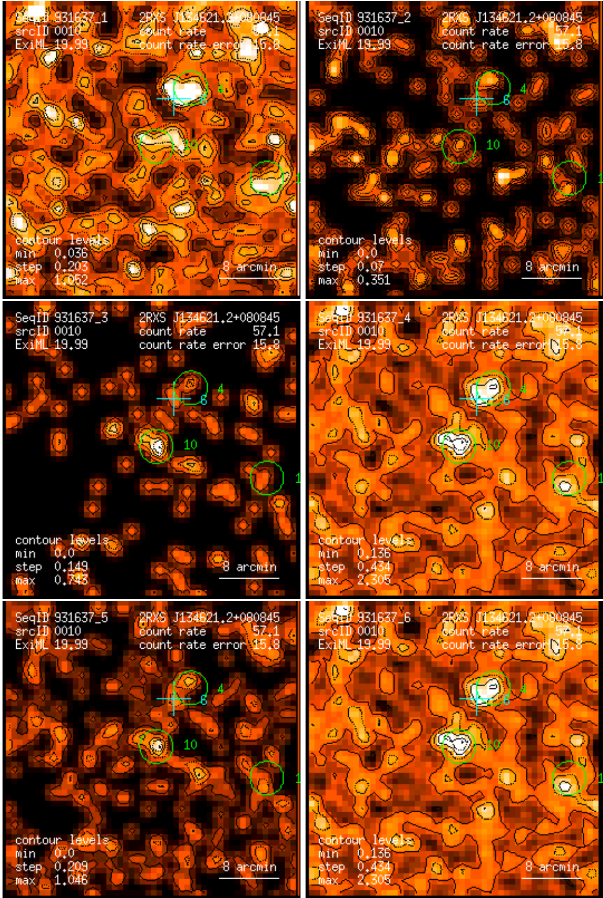
Figure 10: RASS 931637: detection 0010: band rate images, Gaussian filter: (1) PSPC channels 11 – 41, (2) 52 – 90, (3) 91 – 201, (4) 11 – 235, (5) 52 – 201, (6) 11 – 201. Broad band rates in counts/ks. Band rate contour levels in counts/ks/arcmin 2 .
