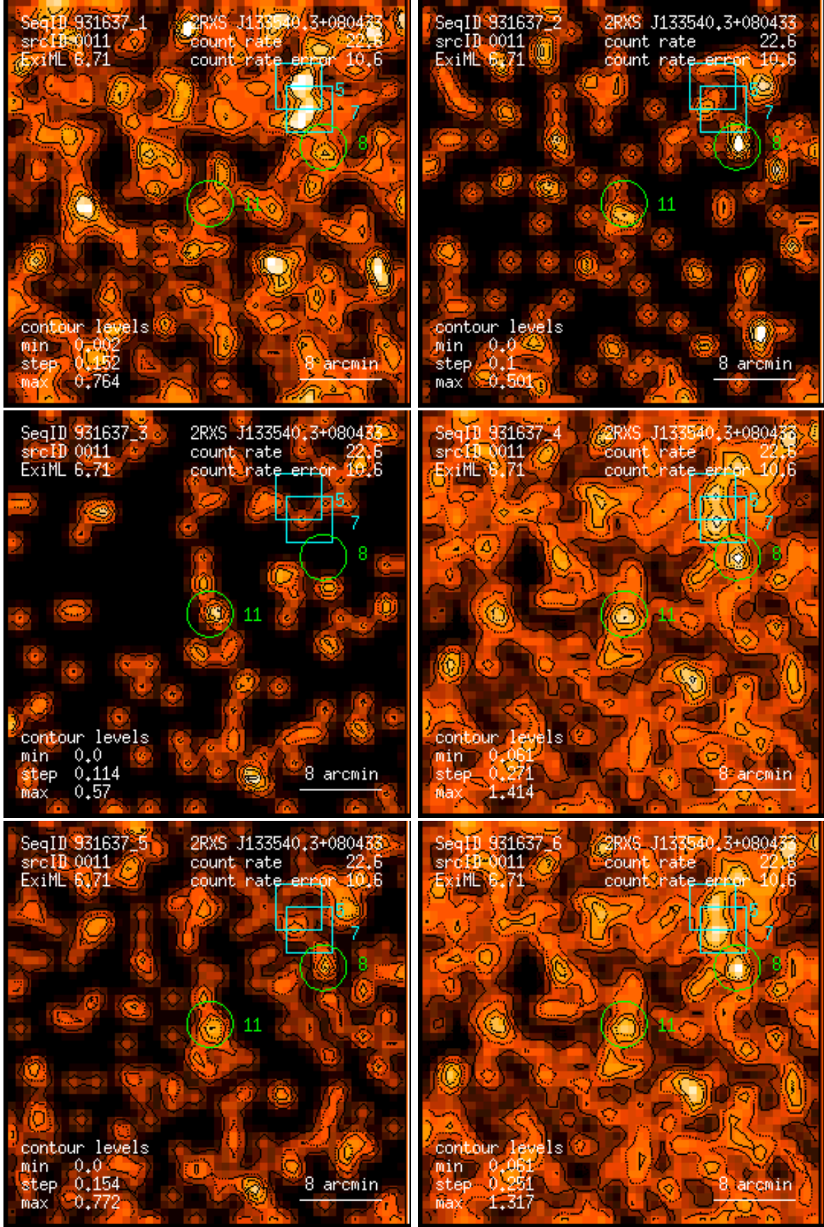
Figure 11: RASS 931637: detection 0011: band rate images, Gaussian filter: (1) PSPC channels 11 – 41, (2) 52 – 90, (3) 91 – 201, (4) 11 – 235, (5) 52 – 201, (6) 11 – 201. Broad band rates in counts/ks. Band rate contour levels in counts/ks/arcmin 2 .
