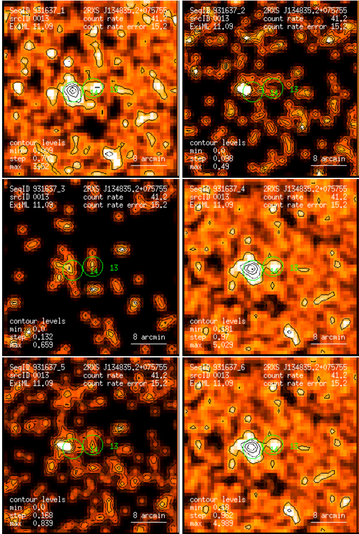
Figure 13: RASS 931637: detection 0013: band rate images, Gaussian filter: (1) PSPC channels 11 – 41, (2) 52 – 90, (3) 91 – 201, (4) 11 – 235, (5) 52 – 201, (6) 11 – 201. Broad band rates in counts/ks. Band rate contour levels in counts/ks/arcmin 2 .
