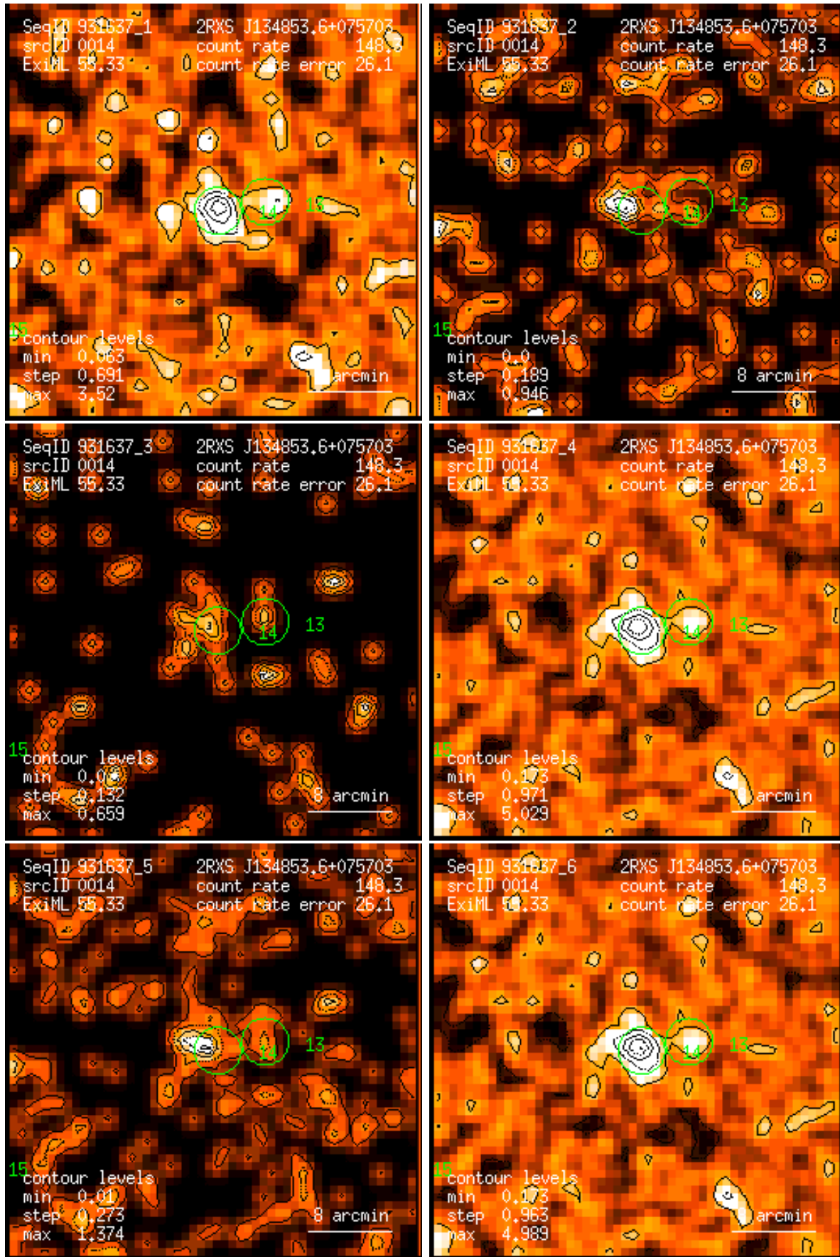
Figure 14: RASS 931637: detection 0014: band rate images, Gaussian filter: (1) PSPC channels 11 – 41, (2) 52 – 90, (3) 91 – 201, (4) 11 – 235, (5) 52 – 201, (6) 11 – 201. Broad band rates in counts/ks. Band rate contour levels in counts/ks/arcmin 2 .
