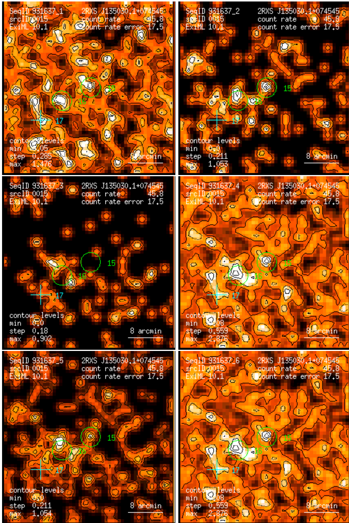
Figure 15: RASS 931637: detection 0015: band rate images, Gaussian filter: (1) PSPC channels 11 – 41, (2) 52 – 90, (3) 91 – 201, (4) 11 – 235, (5) 52 – 201, (6) 11 – 201. Broad band rates in counts/ks. Band rate contour levels in counts/ks/arcmin 2 .
