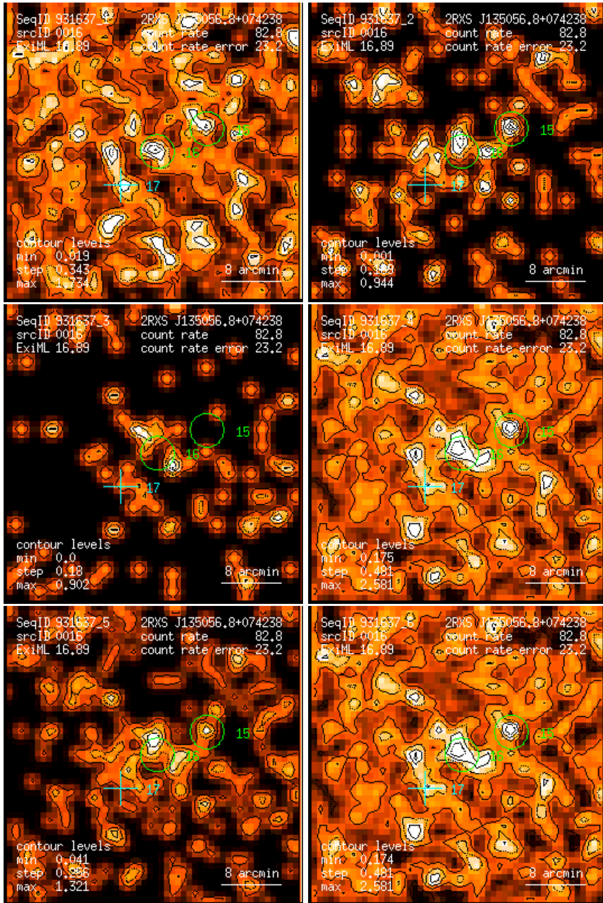
Figure 16: RASS 931637: detection 0016: band rate images, Gaussian filter: (1) PSPC channels 11 – 41, (2) 52 – 90, (3) 91 – 201, (4) 11 – 235, (5) 52 – 201, (6) 11 – 201. Broad band rates in counts/ks. Band rate contour levels in counts/ks/arcmin 2 .
