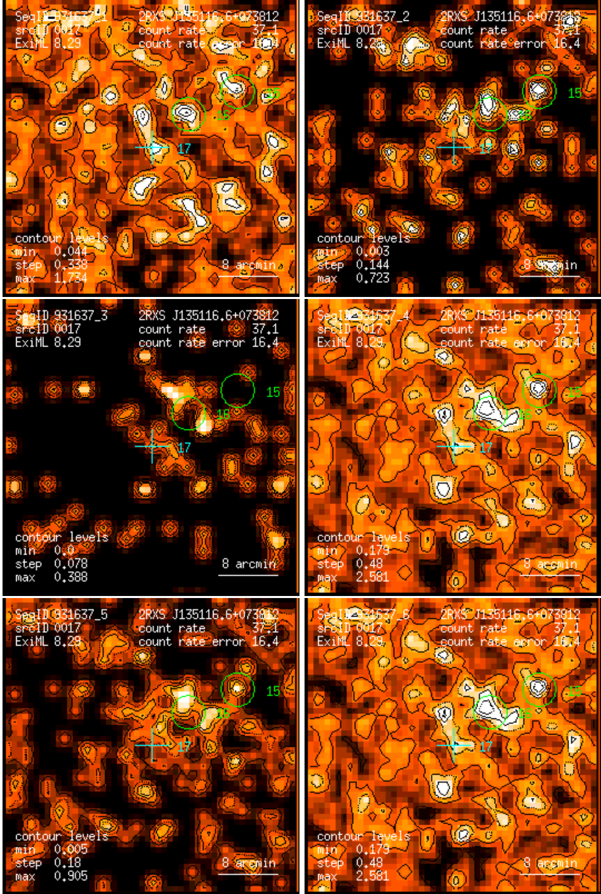
Figure 17: RASS 931637: detection 0017: band rate images, Gaussian filter: (1) PSPC channels 11 – 41, (2) 52 – 90, (3) 91 – 201, (4) 11 – 235, (5) 52 – 201, (6) 11 – 201. Broad band rates in counts/ks. Band rate contour levels in counts/ks/arcmin 2 .
