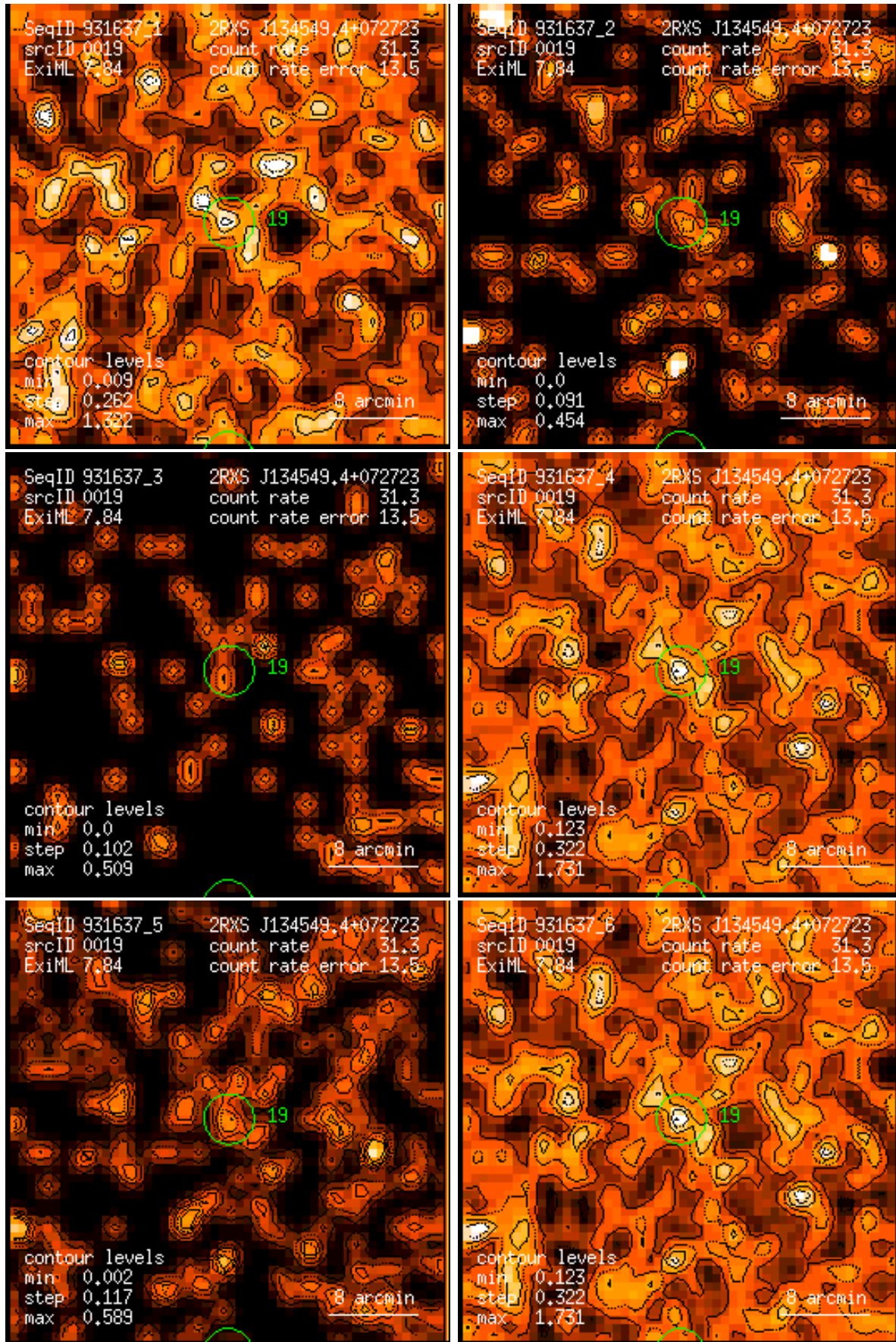
Figure 19: RASS 931637: detection 0019: band rate images, Gaussian filter: (1) PSPC channels 11 – 41, (2) 52 – 90, (3) 91 – 201, (4) 11 – 235, (5) 52 – 201, (6) 11 – 201. Broad band rates in counts/ks. Band rate contour levels in counts/ks/arcmin 2 .
