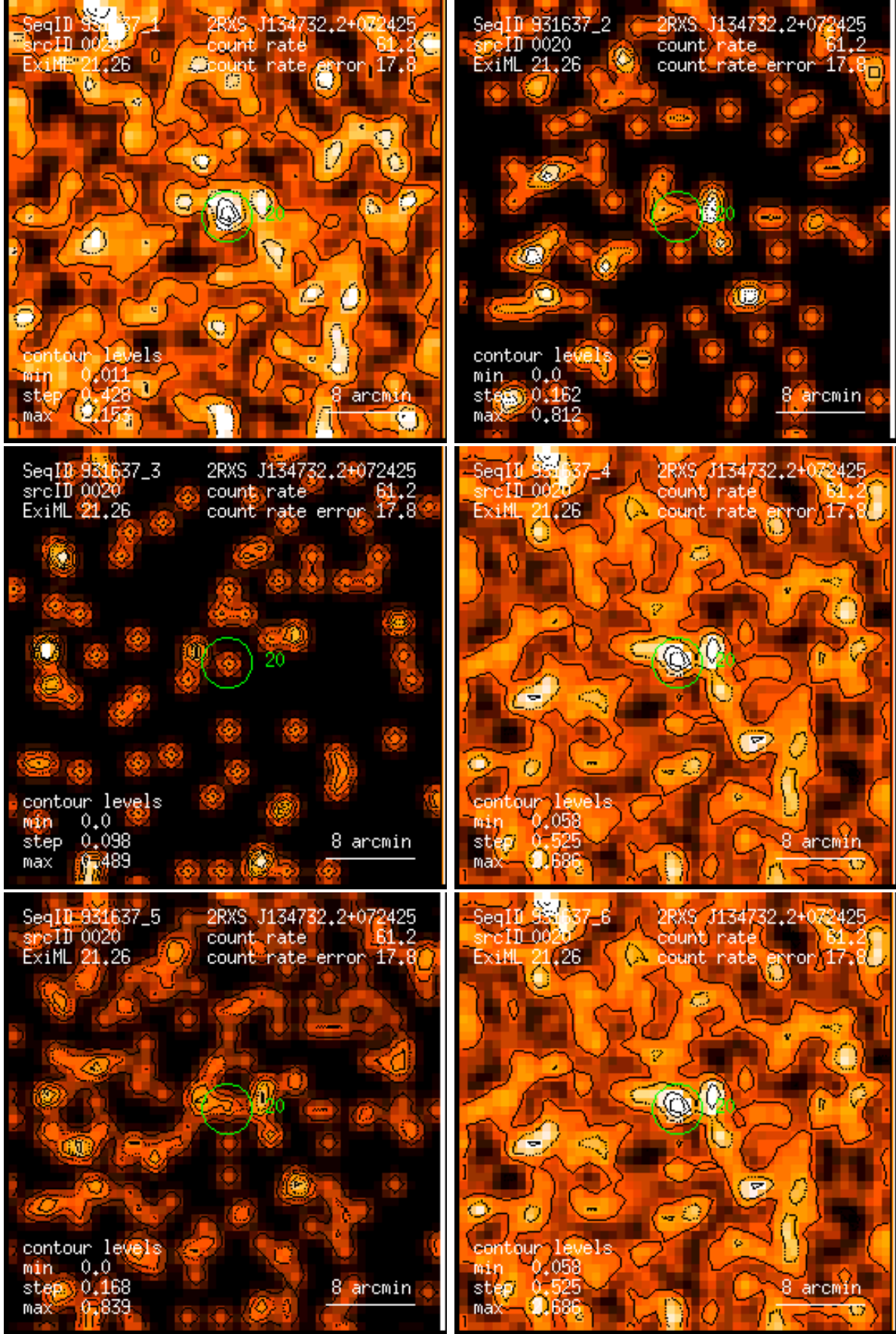
Figure 20: RASS 931637: detection 0020: band rate images, Gaussian filter: (1) PSPC channels 11 – 41, (2) 52 – 90, (3) 91 – 201, (4) 11 – 235, (5) 52 – 201, (6) 11 – 201. Broad band rates in counts/ks. Band rate contour levels in counts/ks/arcmin 2 .
