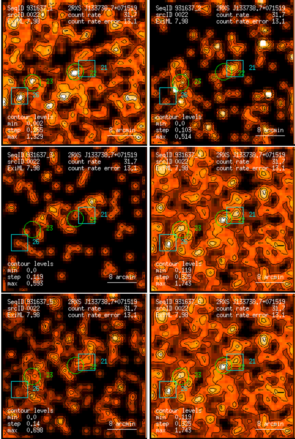
Figure 22: RASS 931637: detection 0022: band rate images, Gaussian filter: (1) PSPC channels 11 – 41, (2) 52 – 90, (3) 91 – 201, (4) 11 – 235, (5) 52 – 201, (6) 11 – 201. Broad band rates in counts/ks. Band rate contour levels in counts/ks/arcmin 2 .
