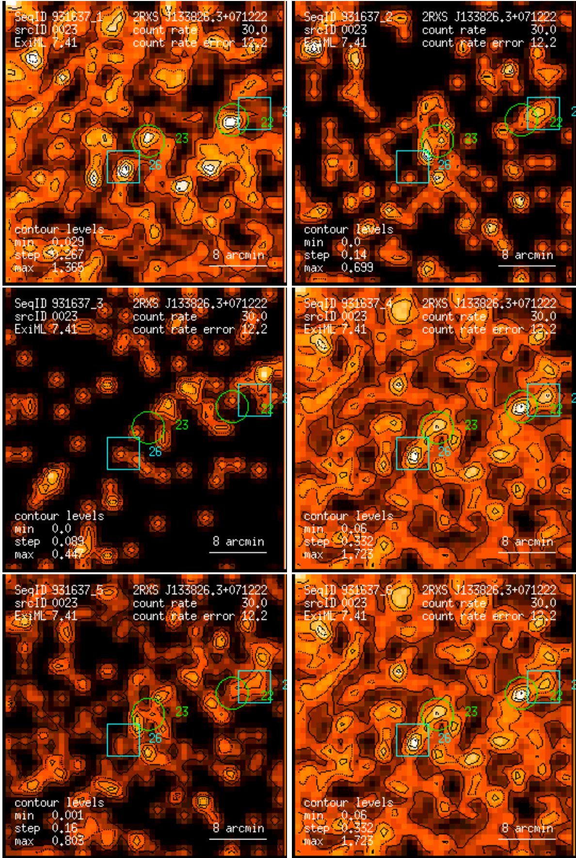
Figure 23: RASS 931637: detection 0023: band rate images, Gaussian filter: (1) PSPC channels 11 – 41, (2) 52 – 90, (3) 91 – 201, (4) 11 – 235, (5) 52 – 201, (6) 11 – 201. Broad band rates in counts/ks. Band rate contour levels in counts/ks/arcmin 2 .
