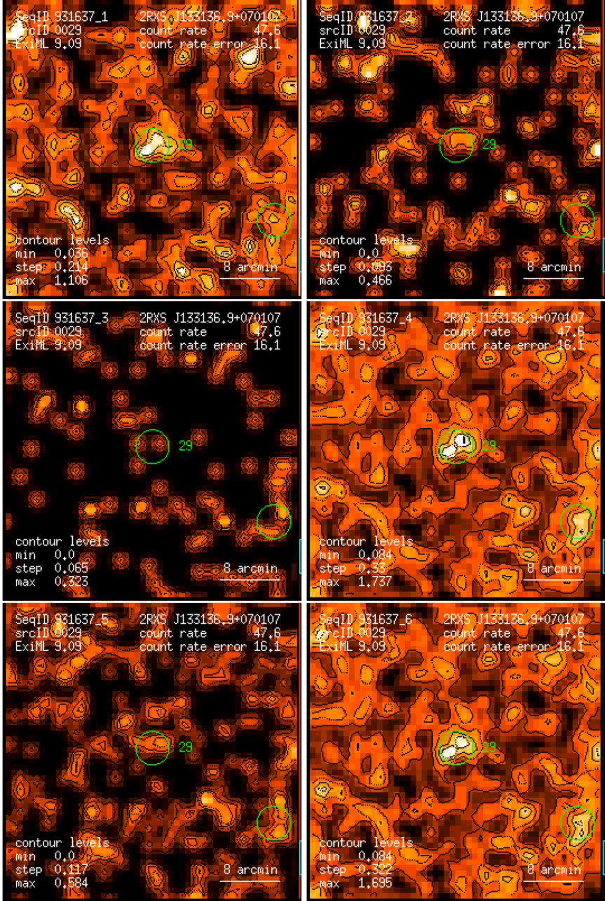
Figure 29: RASS 931637: detection 0029: band rate images, Gaussian filter: (1) PSPC channels 11 – 41, (2) 52 – 90, (3) 91 – 201, (4) 11 – 235, (5) 52 – 201, (6) 11 – 201. Broad band rates in counts/ks. Band rate contour levels in counts/ks/arcmin 2 .
