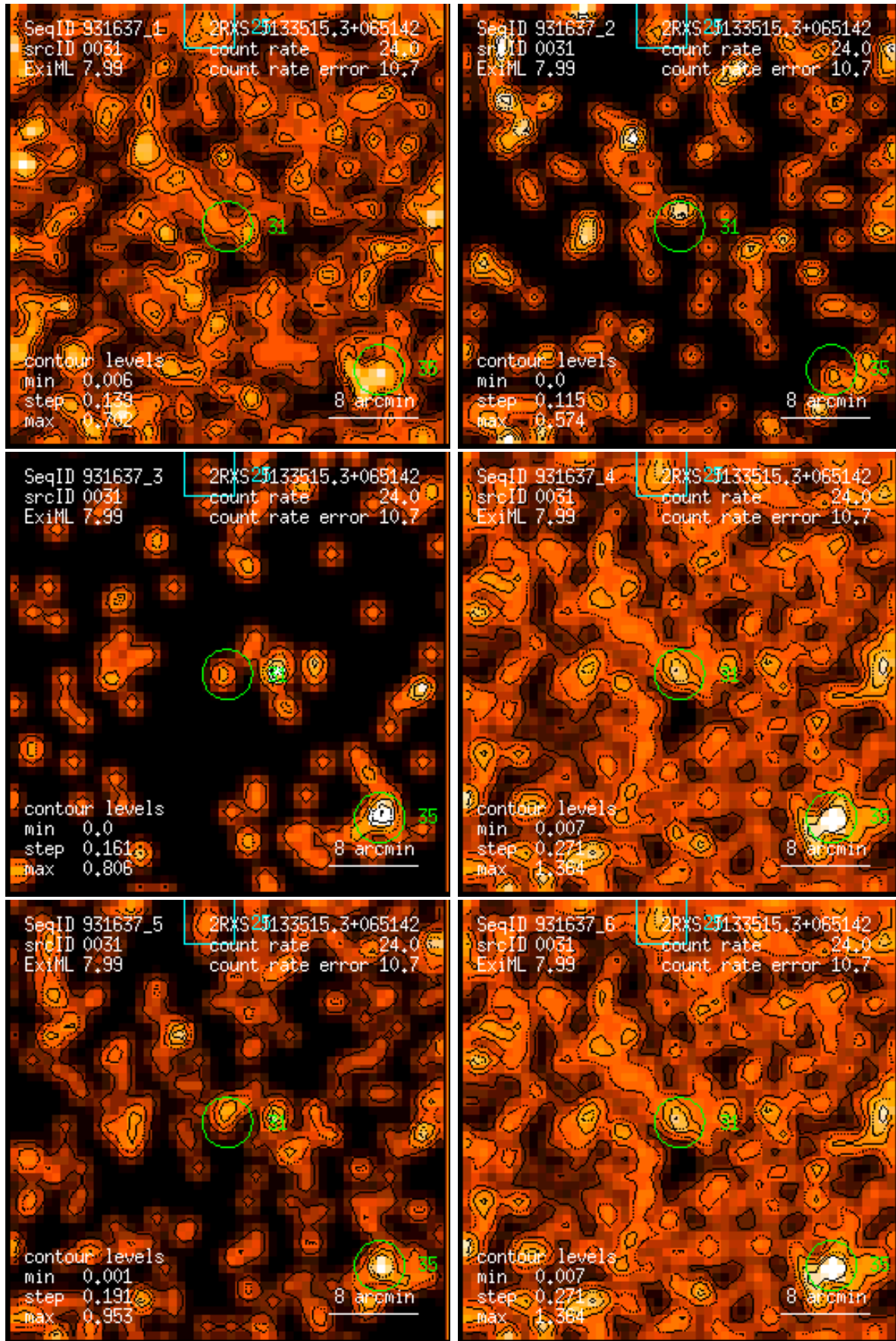
Figure 31: RASS 931637: detection 0031: band rate images, Gaussian filter: (1) PSPC channels 11 – 41, (2) 52 – 90, (3) 91 – 201, (4) 11 – 235, (5) 52 – 201, (6) 11 – 201. Broad band rates in counts/ks. Band rate contour levels in counts/ks/arcmin 2 .
