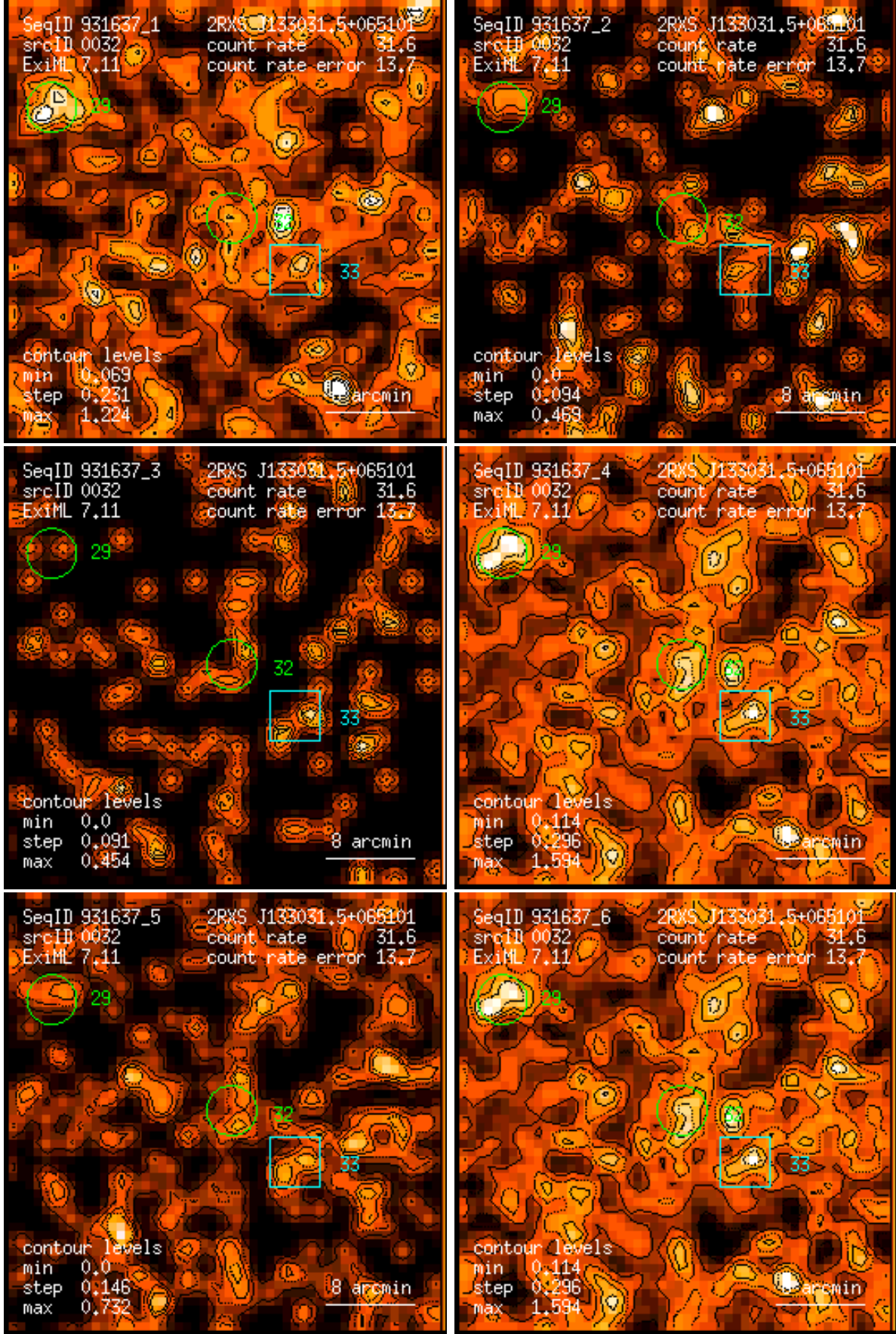
Figure 32: RASS 931637: detection 0032: band rate images, Gaussian filter: (1) PSPC channels 11 – 41, (2) 52 – 90, (3) 91 – 201, (4) 11 – 235, (5) 52 – 201, (6) 11 – 201. Broad band rates in counts/ks. Band rate contour levels in counts/ks/arcmin 2 .
