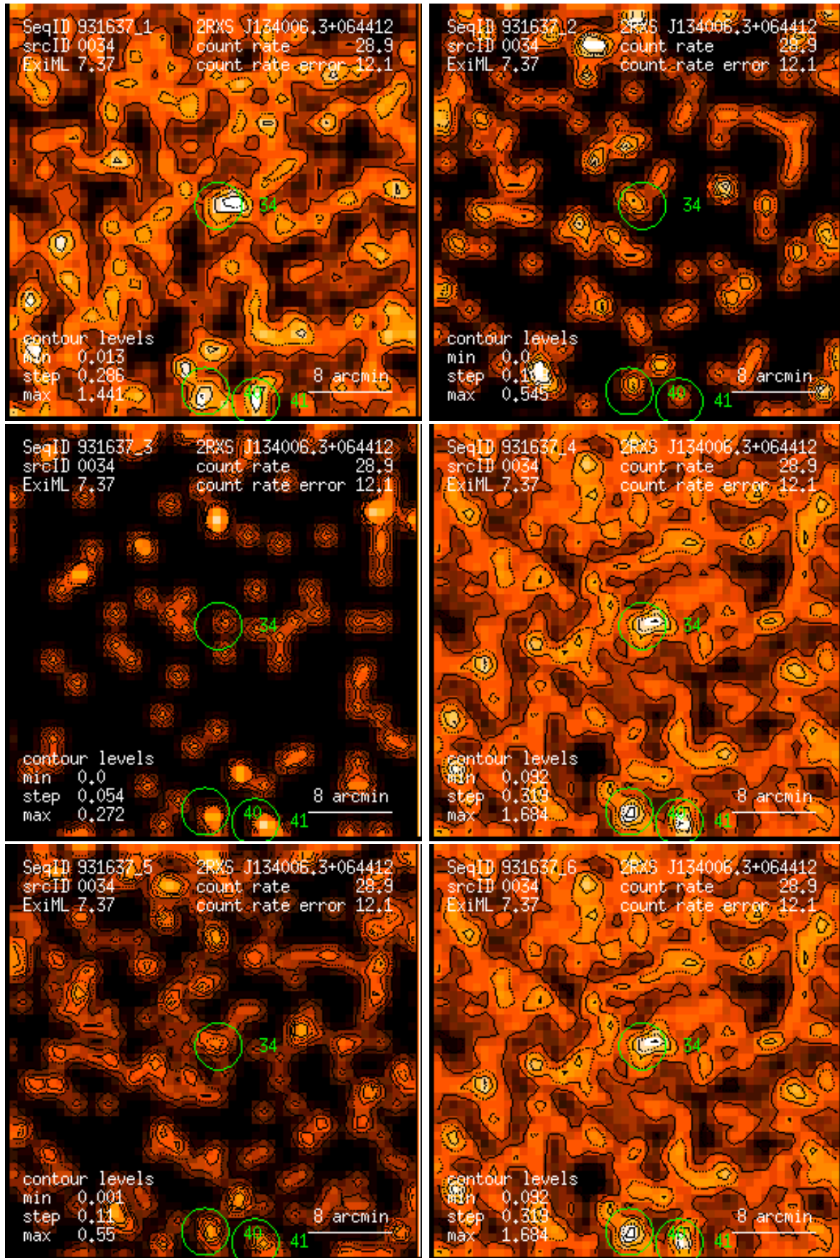
Figure 34: RASS 931637: detection 0034: band rate images, Gaussian filter: (1) PSPC channels 11 – 41, (2) 52 – 90, (3) 91 – 201, (4) 11 – 235, (5) 52 – 201, (6) 11 – 201. Broad band rates in counts/ks. Band rate contour levels in counts/ks/arcmin 2 .
