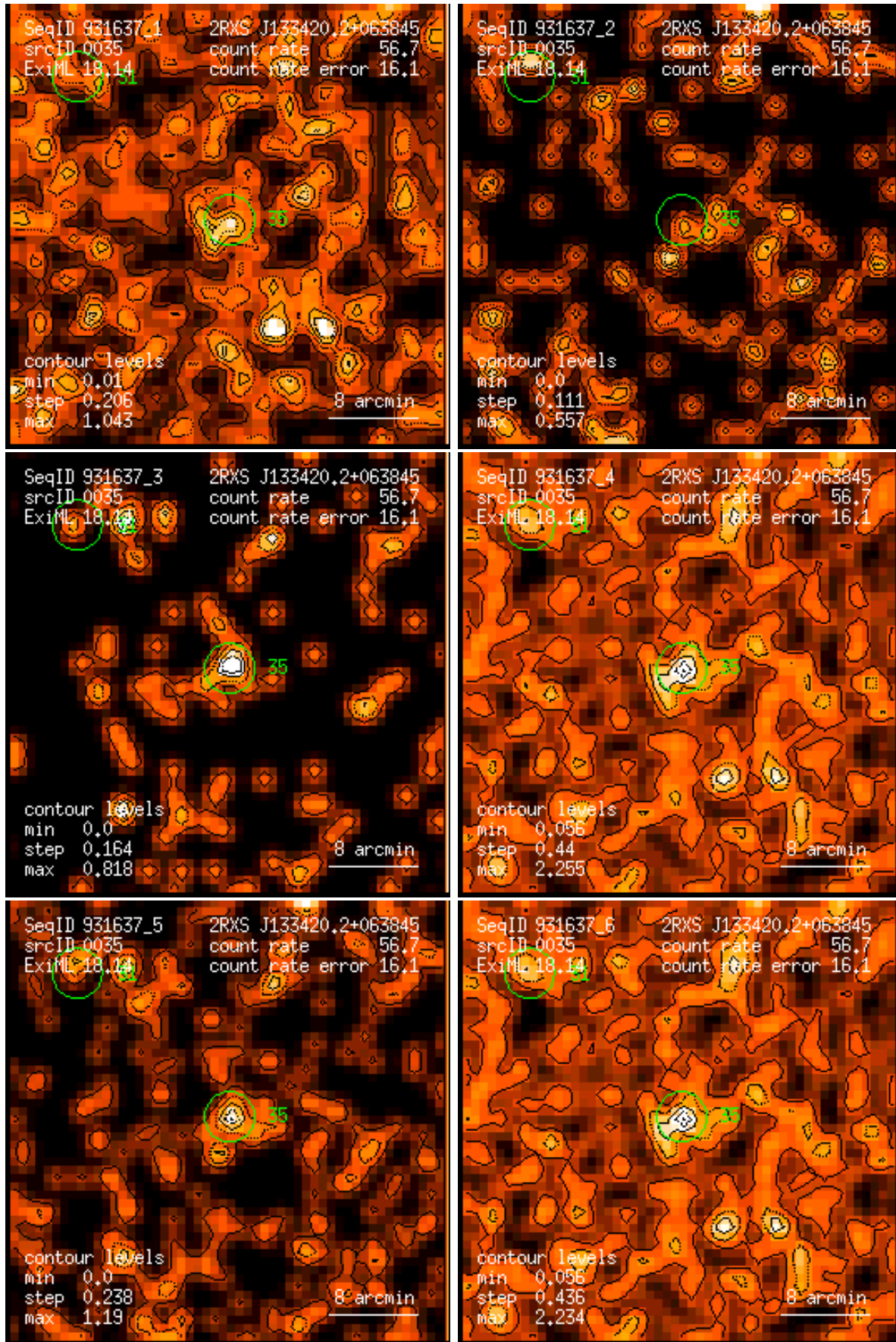
Figure 35: RASS 931637: detection 0035: band rate images, Gaussian filter: (1) PSPC channels 11 – 41, (2) 52 – 90, (3) 91 – 201, (4) 11 – 235, (5) 52 – 201, (6) 11 – 201. Broad band rates in counts/ks. Band rate contour levels in counts/ks/arcmin 2 .
