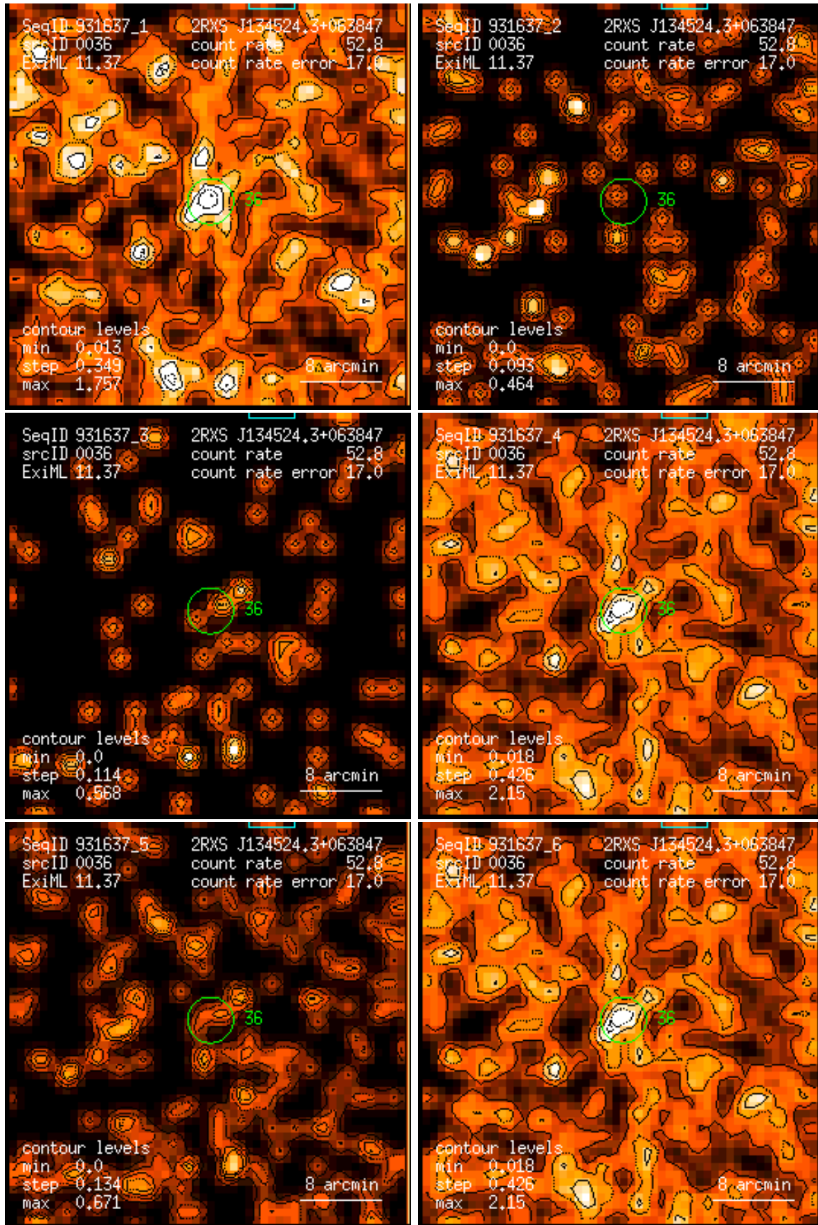
Figure 36: RASS 931637: detection 0036: band rate images, Gaussian filter: (1) PSPC channels 11 – 41, (2) 52 – 90, (3) 91 – 201, (4) 11 – 235, (5) 52 – 201, (6) 11 – 201. Broad band rates in counts/ks. Band rate contour levels in counts/ks/arcmin 2 .
