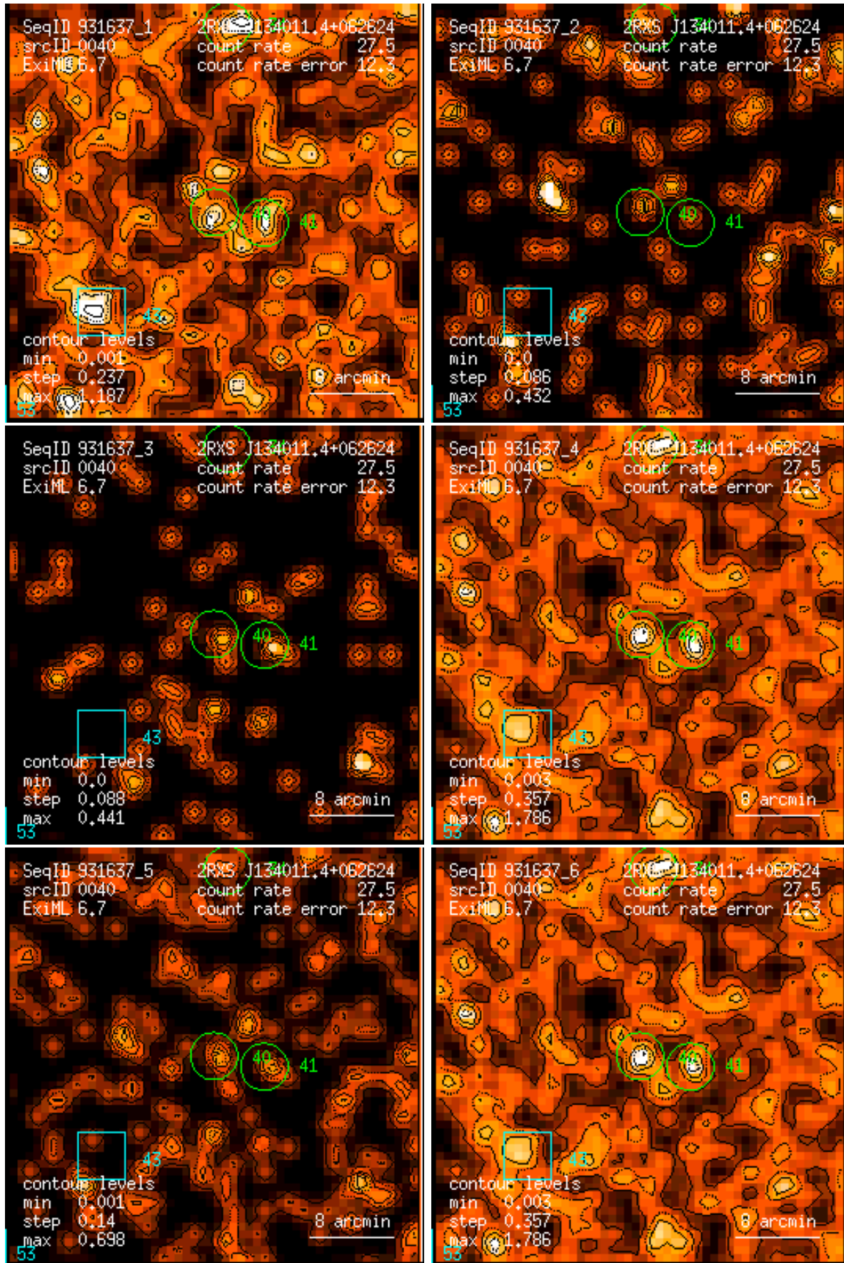
Figure 40: RASS 931637: detection 0040: band rate images, Gaussian filter: (1) PSPC channels 11 – 41, (2) 52 – 90, (3) 91 – 201, (4) 11 – 235, (5) 52 – 201, (6) 11 – 201. Broad band rates in counts/ks. Band rate contour levels in counts/ks/arcmin 2 .
