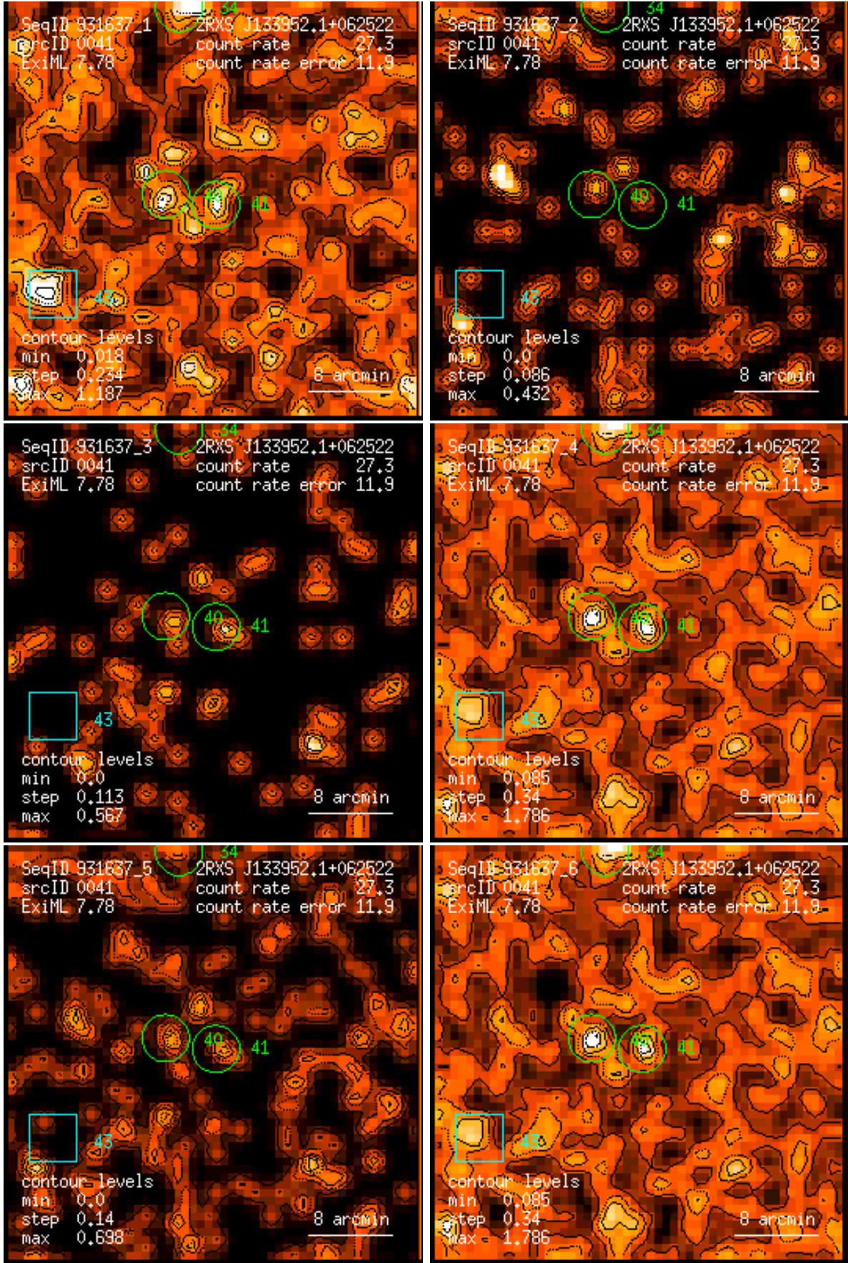
Figure 41: RASS 931637: detection 0041: band rate images, Gaussian filter: (1) PSPC channels 11 – 41, (2) 52 – 90, (3) 91 – 201, (4) 11 – 235, (5) 52 – 201, (6) 11 – 201. Broad band rates in counts/ks. Band rate contour levels in counts/ks/arcmin 2 .
