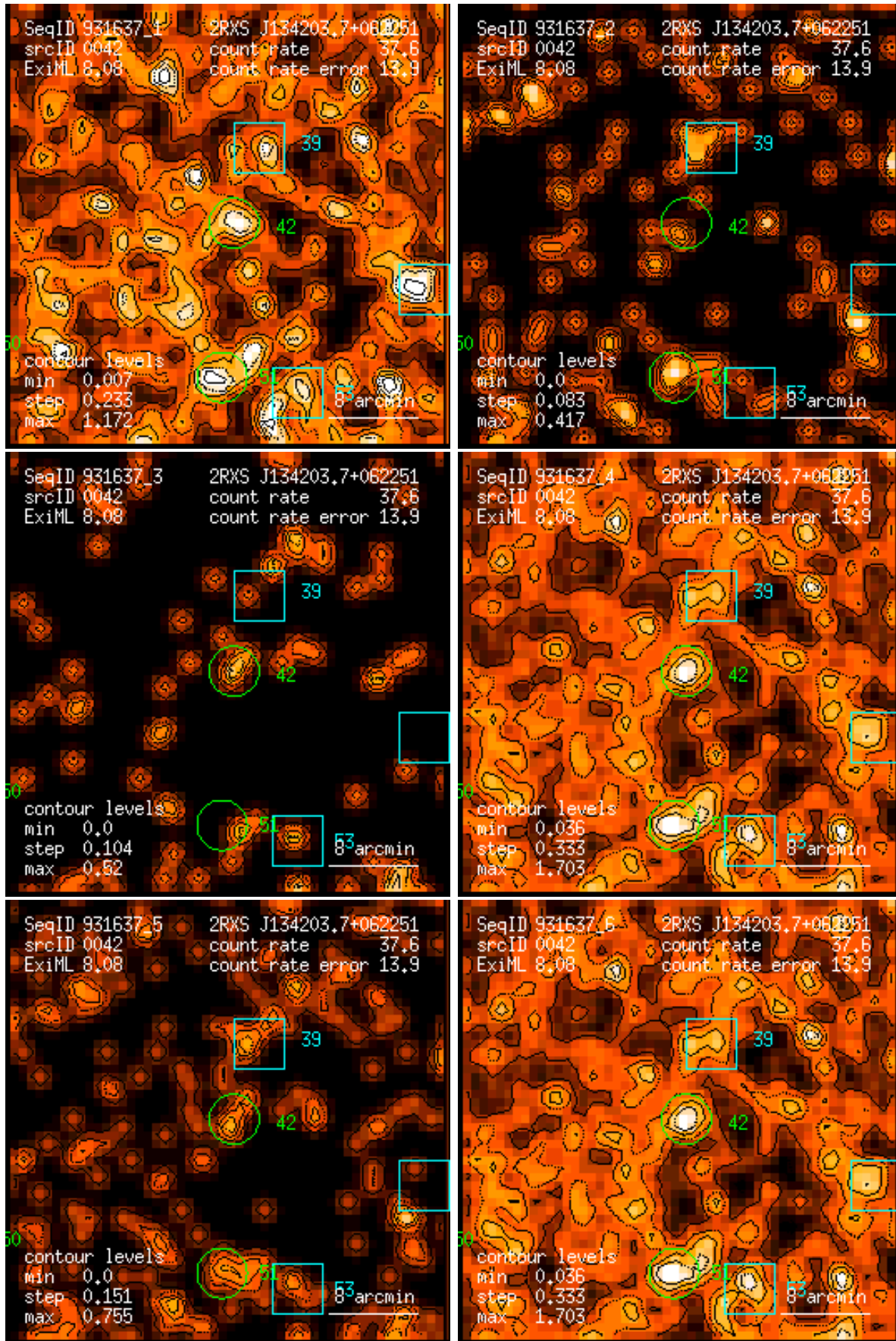
Figure 42: RASS 931637: detection 0042: band rate images, Gaussian filter: (1) PSPC channels 11 – 41, (2) 52 – 90, (3) 91 – 201, (4) 11 – 235, (5) 52 – 201, (6) 11 – 201. Broad band rates in counts/ks. Band rate contour levels in counts/ks/arcmin 2 .
