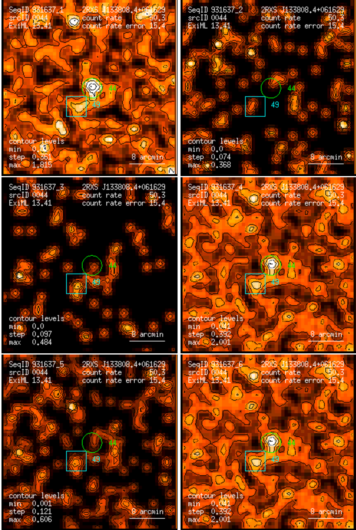
Figure 44: RASS 931637: detection 0044: band rate images, Gaussian filter: (1) PSPC channels 11 – 41, (2) 52 – 90, (3) 91 – 201, (4) 11 – 235, (5) 52 – 201, (6) 11 – 201. Broad band rates in counts/ks. Band rate contour levels in counts/ks/arcmin 2 .
