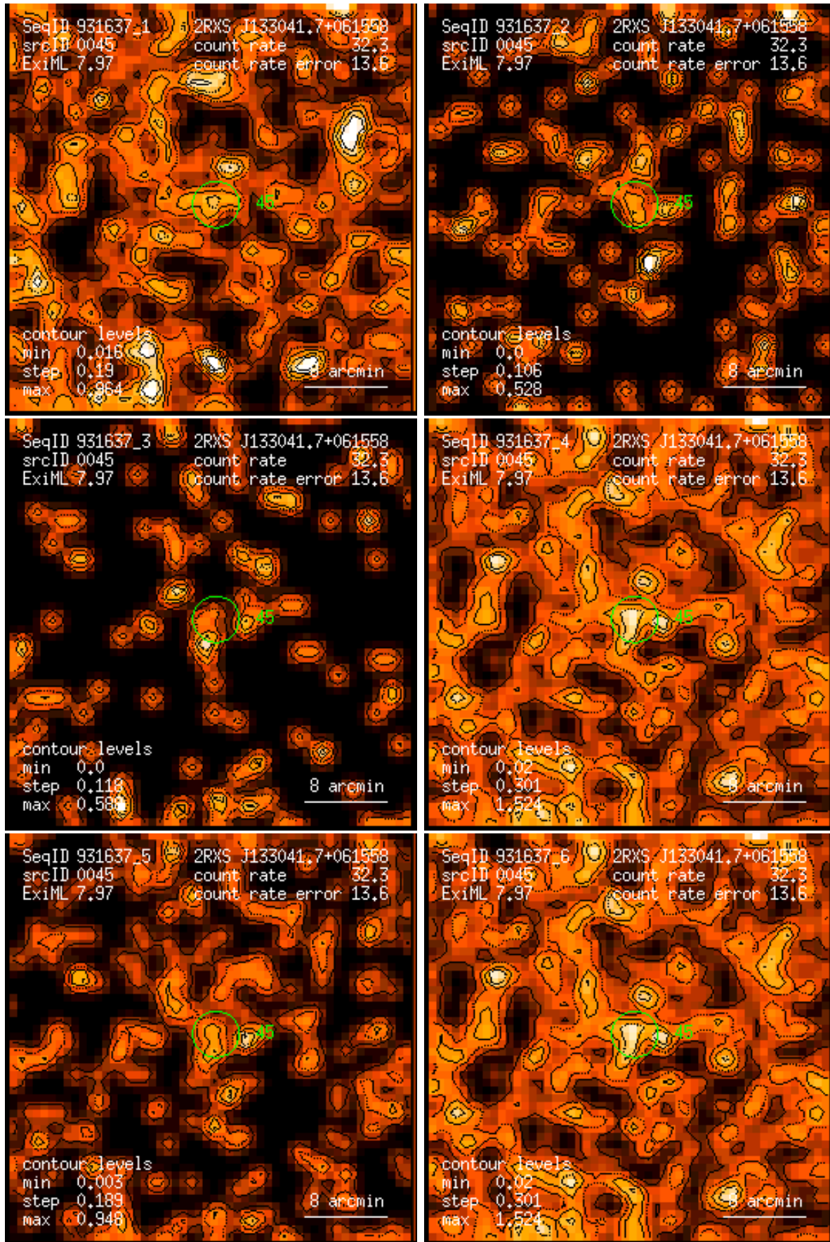
Figure 45: RASS 931637: detection 0045: band rate images, Gaussian filter: (1) PSPC channels 11 – 41, (2) 52 – 90, (3) 91 – 201, (4) 11 – 235, (5) 52 – 201, (6) 11 – 201. Broad band rates in counts/ks. Band rate contour levels in counts/ks/arcmin 2 .
