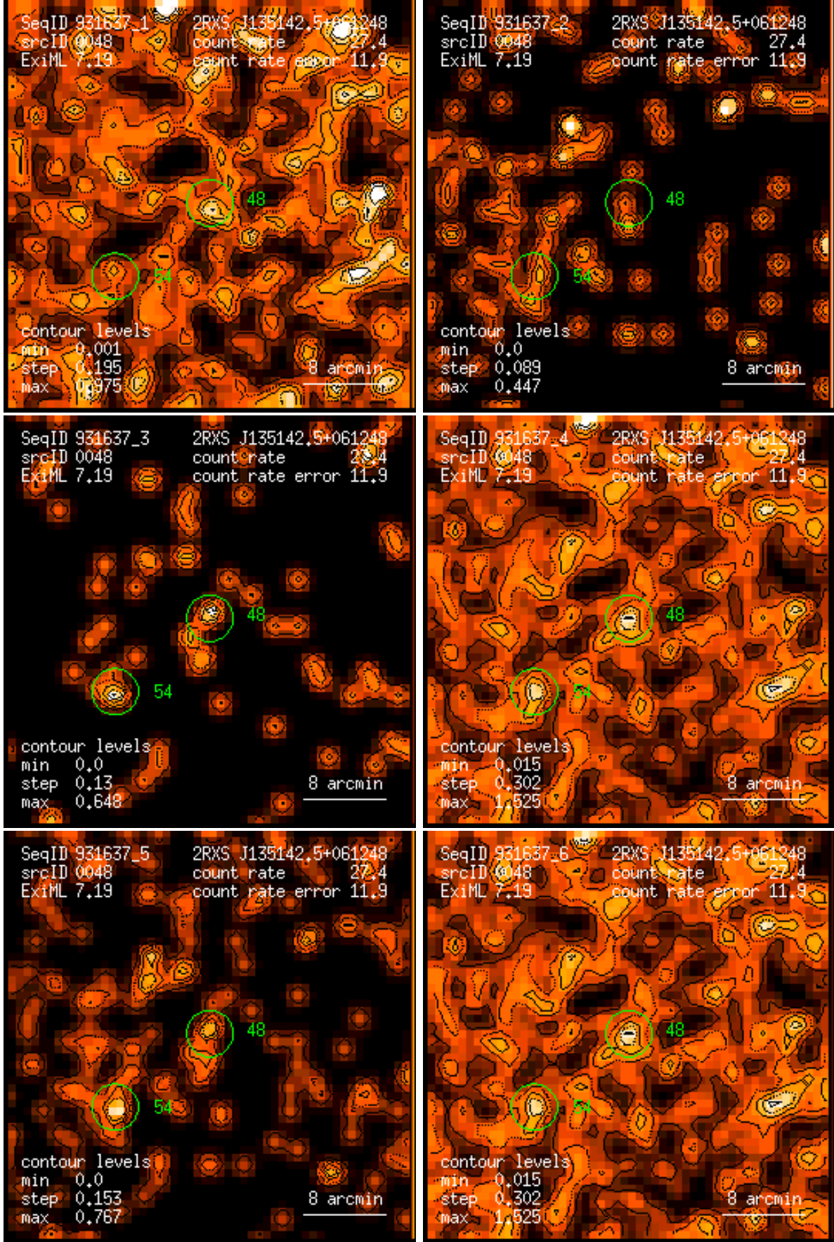
Figure 48: RASS 931637: detection 0048: band rate images, Gaussian filter: (1) PSPC channels 11 – 41, (2) 52 – 90, (3) 91 – 201, (4) 11 – 235, (5) 52 – 201, (6) 11 – 201. Broad band rates in counts/ks. Band rate contour levels in counts/ks/arcmin 2 .
