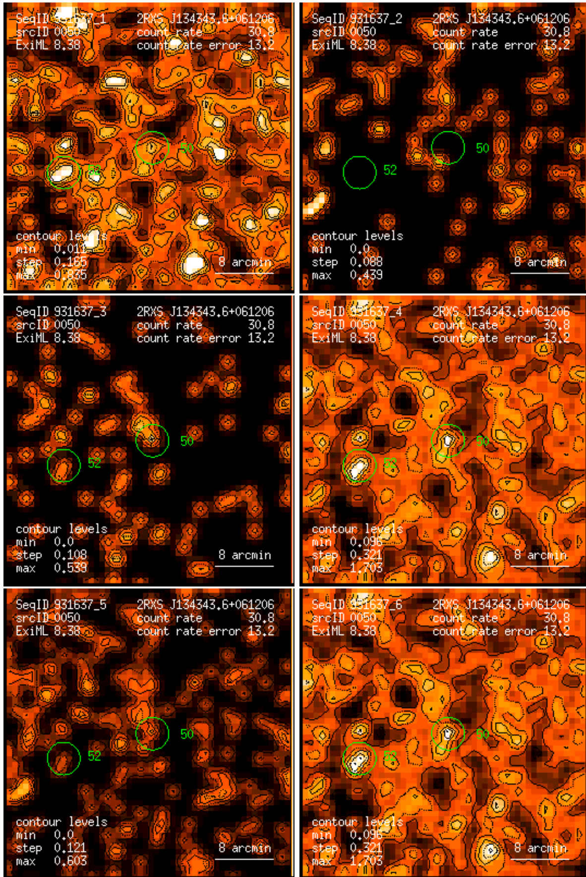
Figure 50: RASS 931637: detection 0050: band rate images, Gaussian filter: (1) PSPC channels 11 – 41, (2) 52 – 90, (3) 91 – 201, (4) 11 – 235, (5) 52 – 201, (6) 11 – 201. Broad band rates in counts/ks. Band rate contour levels in counts/ks/arcmin 2 .
