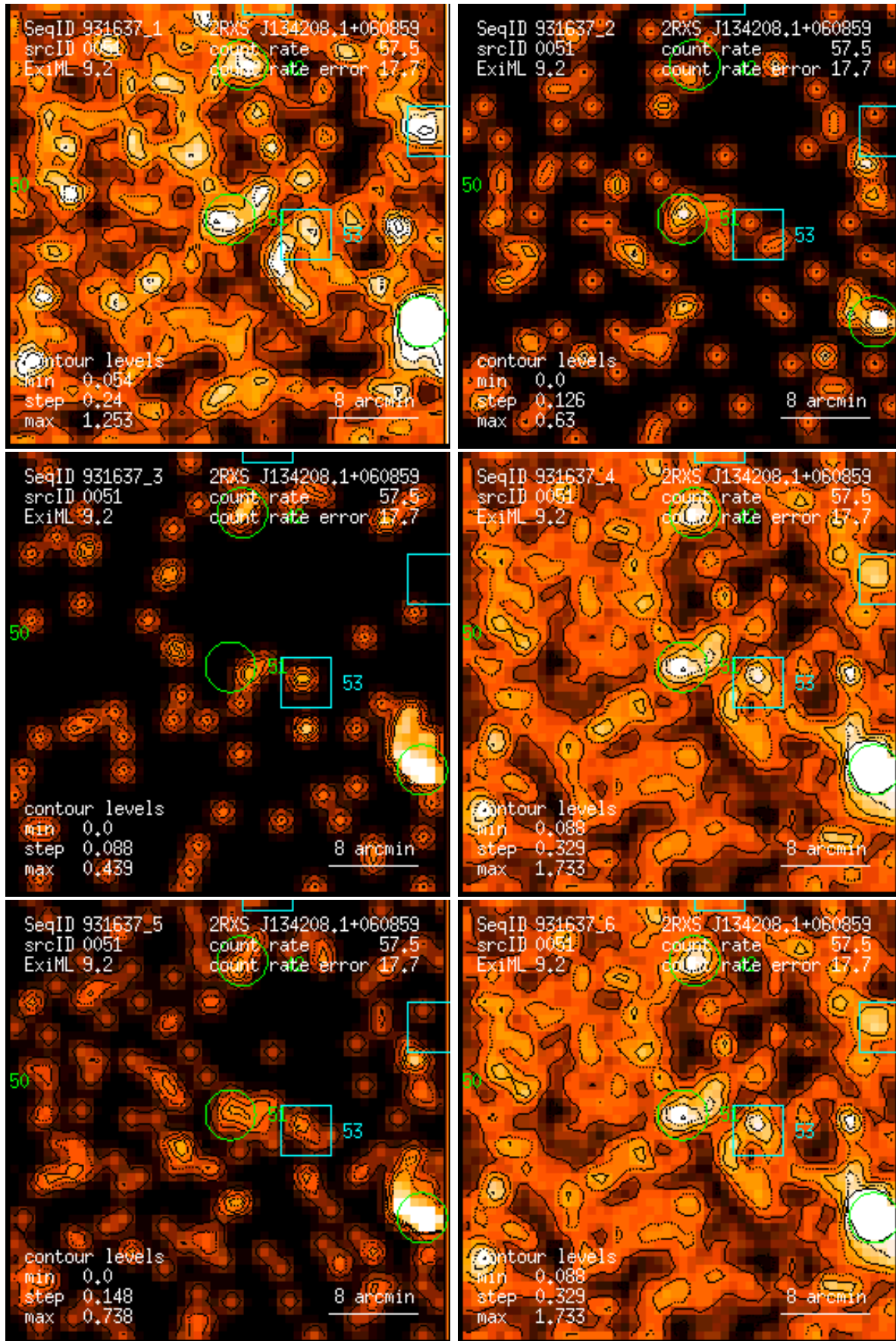
Figure 51: RASS 931637: detection 0051: band rate images, Gaussian filter: (1) PSPC channels 11 – 41, (2) 52 – 90, (3) 91 – 201, (4) 11 – 235, (5) 52 – 201, (6) 11 – 201. Broad band rates in counts/ks. Band rate contour levels in counts/ks/arcmin 2 .
