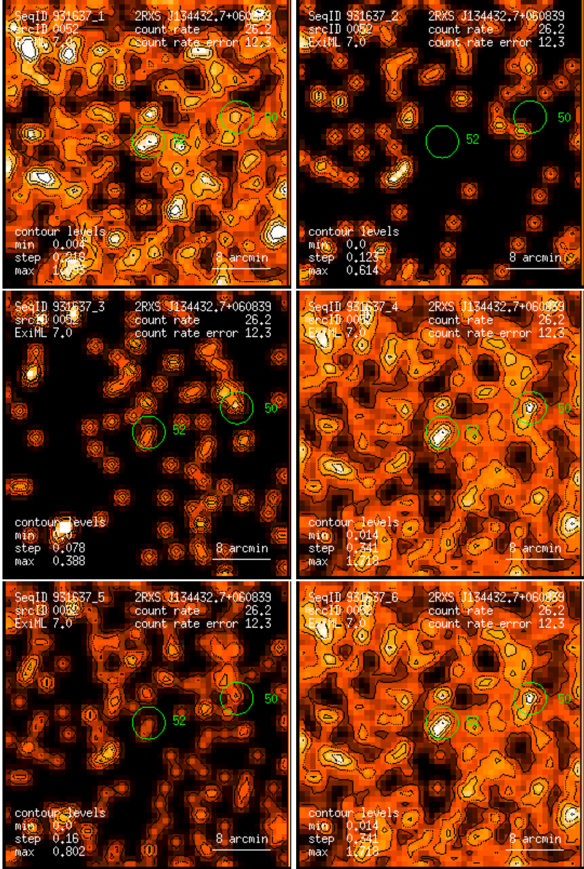
Figure 52: RASS 931637: detection 0052: band rate images, Gaussian filter: (1) PSPC channels 11 – 41, (2) 52 – 90, (3) 91 – 201, (4) 11 – 235, (5) 52 – 201, (6) 11 – 201. Broad band rates in counts/ks. Band rate contour levels in counts/ks/arcmin 2 .
