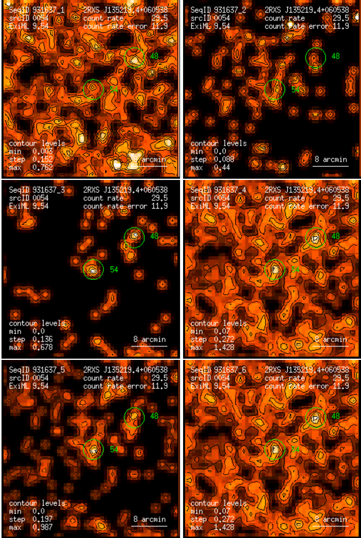
Figure 54: RASS 931637: detection 0054: band rate images, Gaussian filter: (1) PSPC channels 11 – 41, (2) 52 – 90, (3) 91 – 201, (4) 11 – 235, (5) 52 – 201, (6) 11 – 201. Broad band rates in counts/ks. Band rate contour levels in counts/ks/arcmin 2 .
