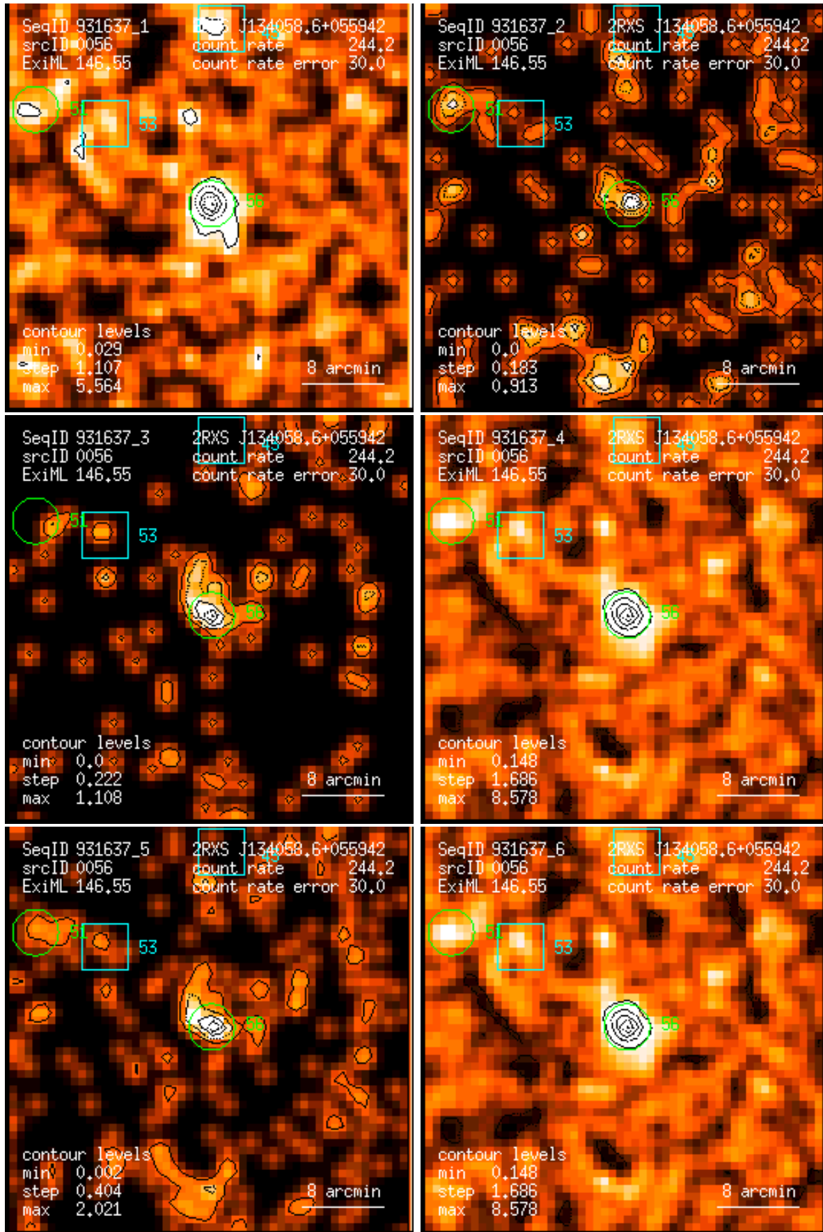
Figure 56: RASS 931637: detection 0056: band rate images, Gaussian filter: (1) PSPC channels 11 – 41, (2) 52 – 90, (3) 91 – 201, (4) 11 – 235, (5) 52 – 201, (6) 11 – 201. Broad band rates in counts/ks. Band rate contour levels in counts/ks/arcmin 2 .
