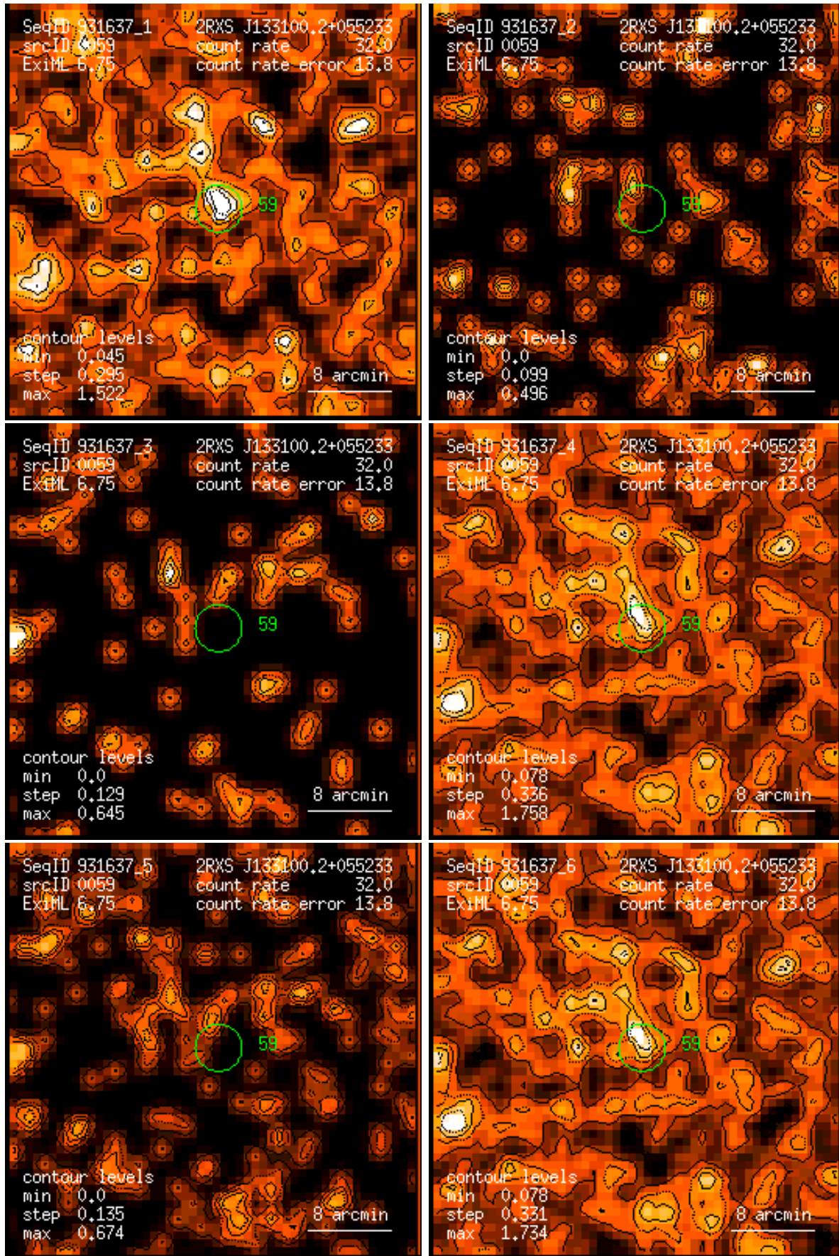
Figure 59: RASS 931637: detection 0059: band rate images, Gaussian filter: (1) PSPC channels 11 – 41, (2) 52 – 90, (3) 91 – 201, (4) 11 – 235, (5) 52 – 201, (6) 11 – 201. Broad band rates in counts/ks. Band rate contour levels in counts/ks/arcmin 2 .
