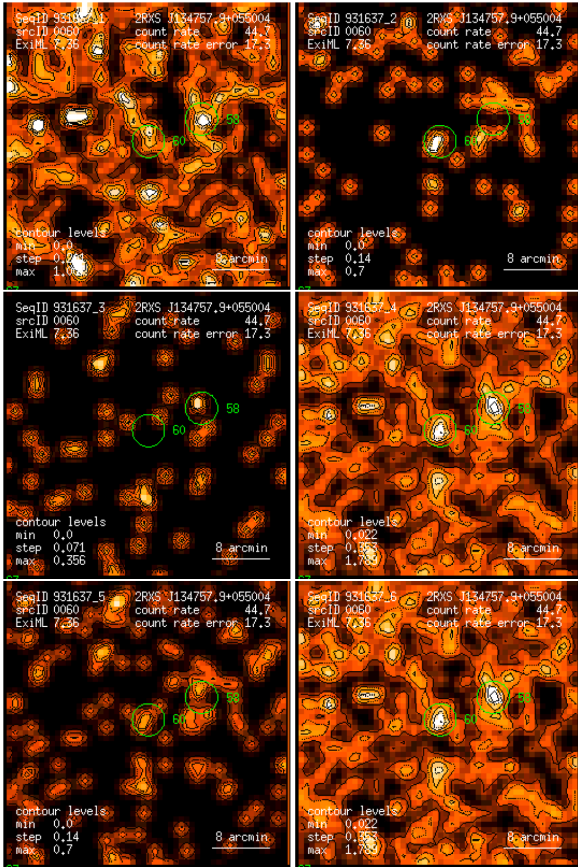
Figure 60: RASS 931637: detection 0060: band rate images, Gaussian filter: (1) PSPC channels 11 – 41, (2) 52 – 90, (3) 91 – 201, (4) 11 – 235, (5) 52 – 201, (6) 11 – 201. Broad band rates in counts/ks. Band rate contour levels in counts/ks/arcmin 2 .
