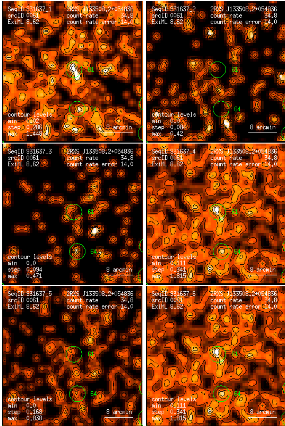
Figure 61: RASS 931637: detection 0061: band rate images, Gaussian filter: (1) PSPC channels 11 – 41, (2) 52 – 90, (3) 91 – 201, (4) 11 – 235, (5) 52 – 201, (6) 11 – 201. Broad band rates in counts/ks. Band rate contour levels in counts/ks/arcmin 2 .
