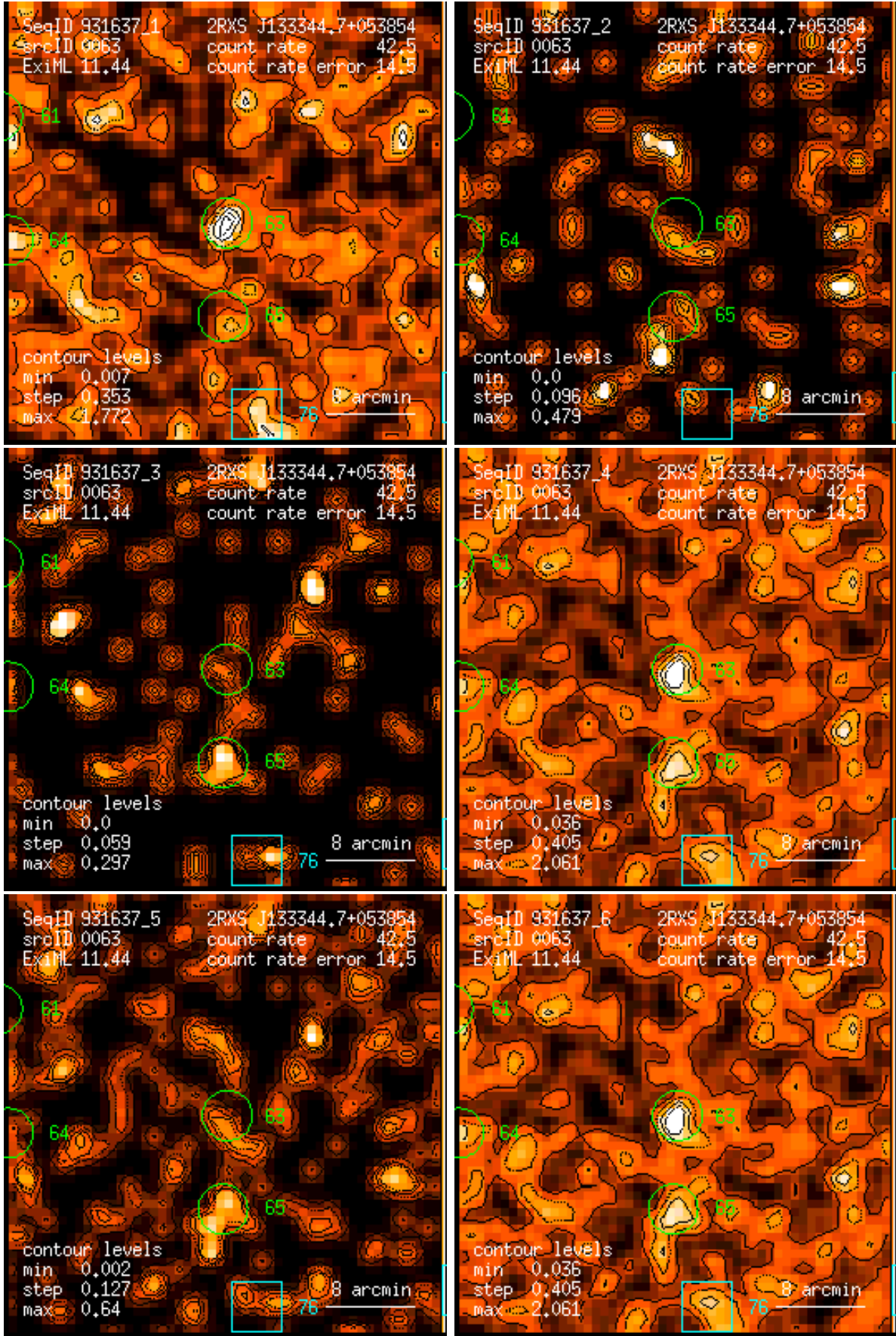
Figure 63: RASS 931637: detection 0063: band rate images, Gaussian filter: (1) PSPC channels 11 – 41, (2) 52 – 90, (3) 91 – 201, (4) 11 – 235, (5) 52 – 201, (6) 11 – 201. Broad band rates in counts/ks. Band rate contour levels in counts/ks/arcmin 2 .
