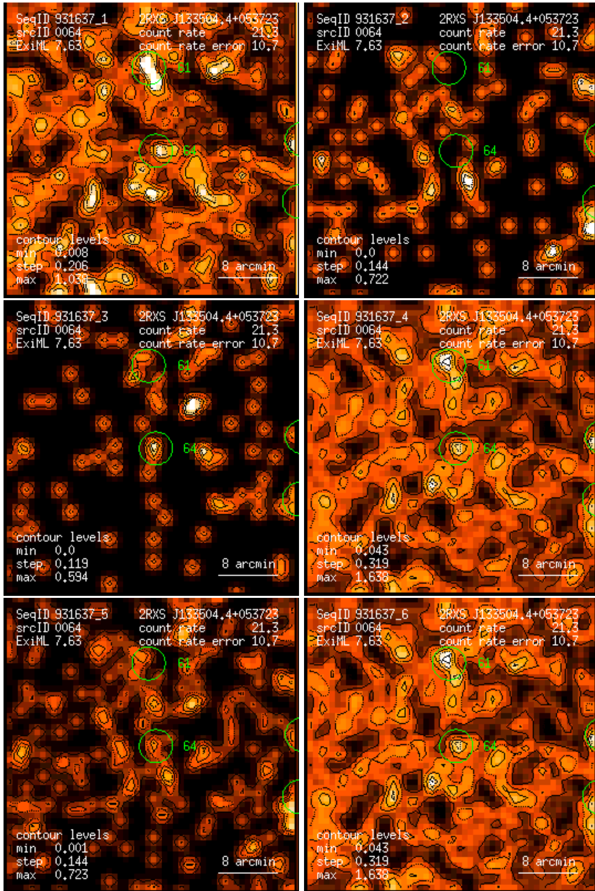
Figure 64: RASS 931637: detection 0064: band rate images, Gaussian filter: (1) PSPC channels 11 – 41, (2) 52 – 90, (3) 91 – 201, (4) 11 – 235, (5) 52 – 201, (6) 11 – 201. Broad band rates in counts/ks. Band rate contour levels in counts/ks/arcmin 2 .
