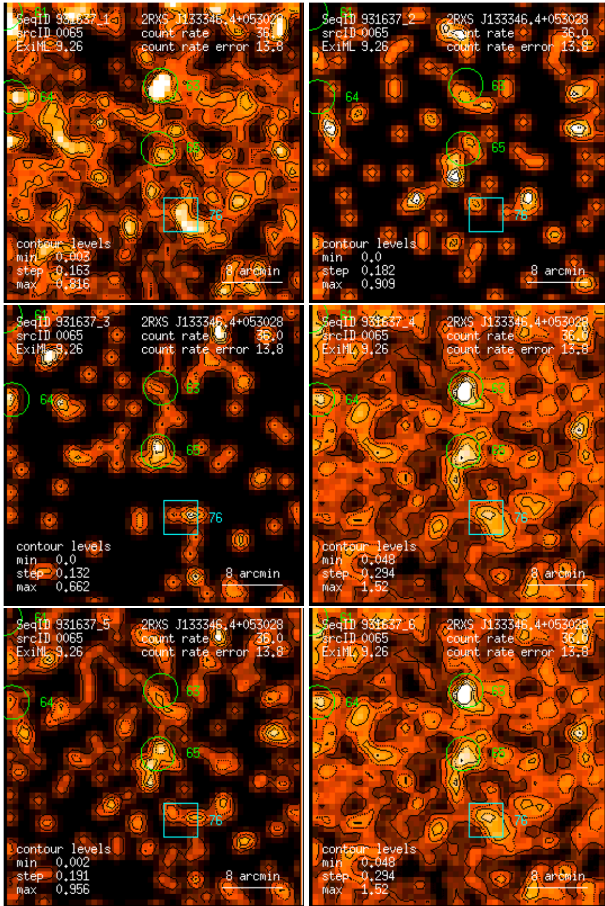
Figure 65: RASS 931637: detection 0065: band rate images, Gaussian filter: (1) PSPC channels 11 – 41, (2) 52 – 90, (3) 91 – 201, (4) 11 – 235, (5) 52 – 201, (6) 11 – 201. Broad band rates in counts/ks. Band rate contour levels in counts/ks/arcmin 2 .
