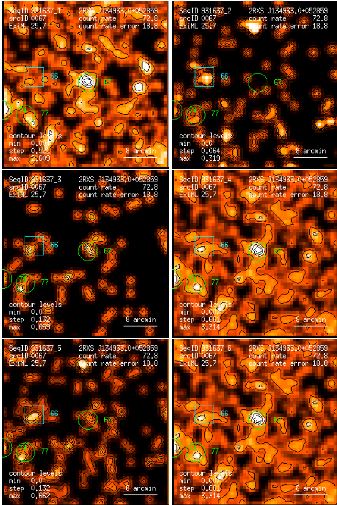
Figure 67: RASS 931637: detection 0067: band rate images, Gaussian filter: (1) PSPC channels 11 – 41, (2) 52 – 90, (3) 91 – 201, (4) 11 – 235, (5) 52 – 201, (6) 11 – 201. Broad band rates in counts/ks. Band rate contour levels in counts/ks/arcmin 2 .
