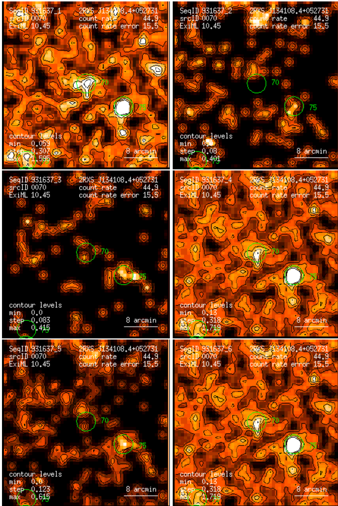
Figure 70: RASS 931637: detection 0070: band rate images, Gaussian filter: (1) PSPC channels 11 – 41, (2) 52 – 90, (3) 91 – 201, (4) 11 – 235, (5) 52 – 201, (6) 11 – 201. Broad band rates in counts/ks. Band rate contour levels in counts/ks/arcmin 2 .
