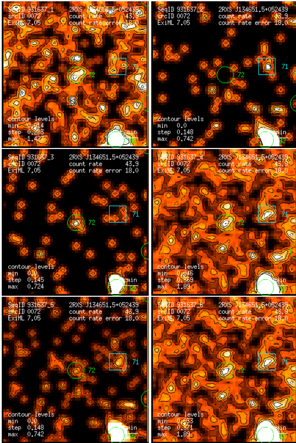
Figure 72: RASS 931637: detection 0072: band rate images, Gaussian filter: (1) PSPC channels 11 – 41, (2) 52 – 90, (3) 91 – 201, (4) 11 – 235, (5) 52 – 201, (6) 11 – 201. Broad band rates in counts/ks. Band rate contour levels in counts/ks/arcmin 2 .
