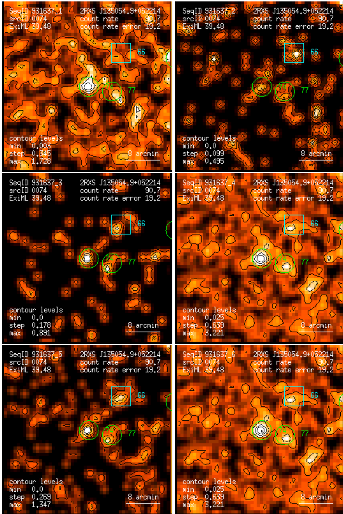
Figure 74: RASS 931637: detection 0074: band rate images, Gaussian filter: (1) PSPC channels 11 – 41, (2) 52 – 90, (3) 91 – 201, (4) 11 – 235, (5) 52 – 201, (6) 11 – 201. Broad band rates in counts/ks. Band rate contour levels in counts/ks/arcmin 2 .
