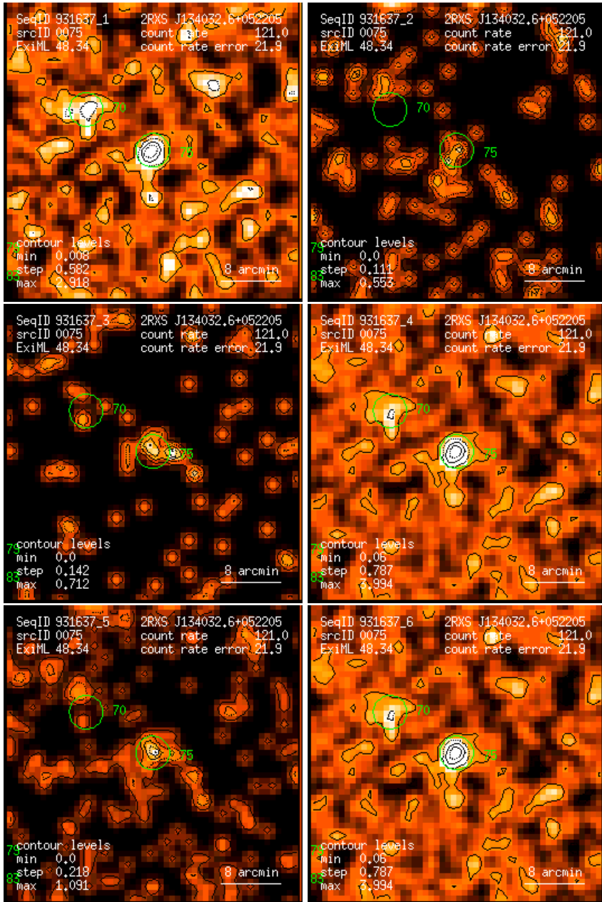
Figure 75: RASS 931637: detection 0075: band rate images, Gaussian filter: (1) PSPC channels 11 – 41, (2) 52 – 90, (3) 91 – 201, (4) 11 – 235, (5) 52 – 201, (6) 11 – 201. Broad band rates in counts/ks. Band rate contour levels in counts/ks/arcmin 2 .
